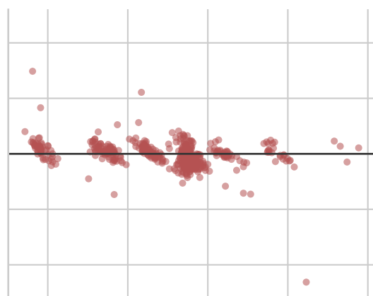
Raw FPLS
