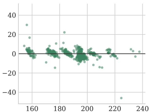
Arnoldi FPLS
