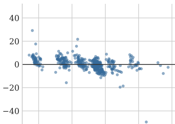
CG-FPLS
