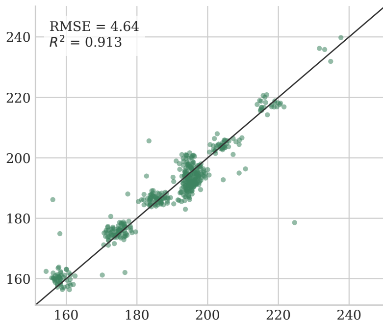
Arnoldi FPLS
