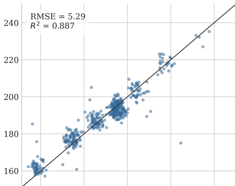
Arnoldi FPLS
