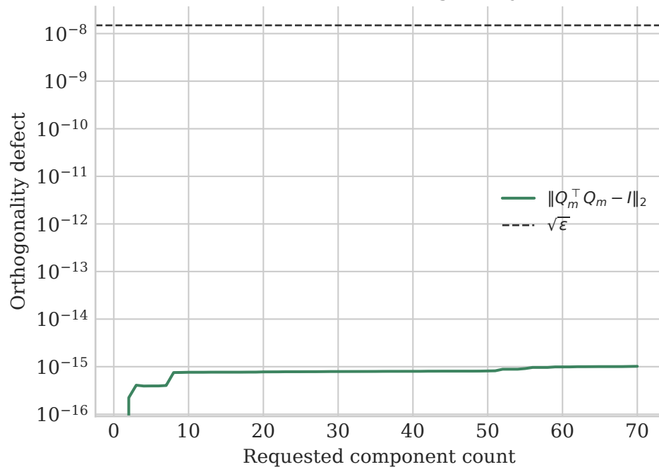
Arnoldi basis orthogonality
