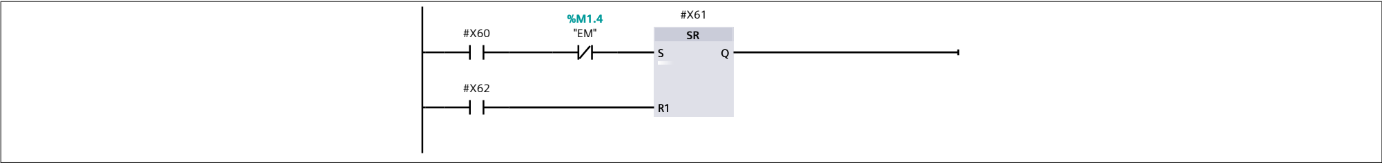
Network 3:
