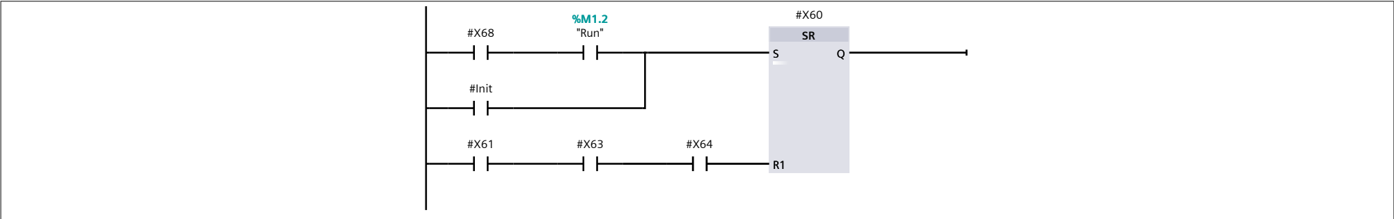
Network 2:
