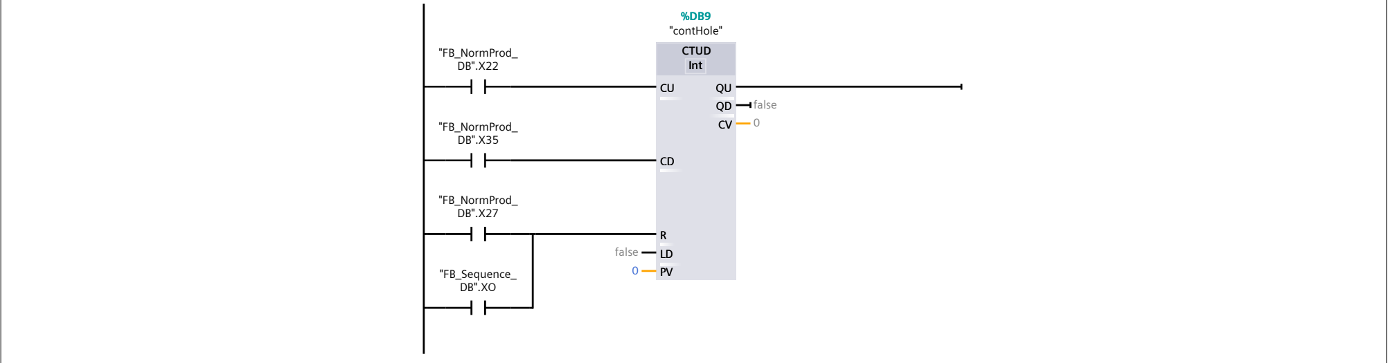
Network 5:
