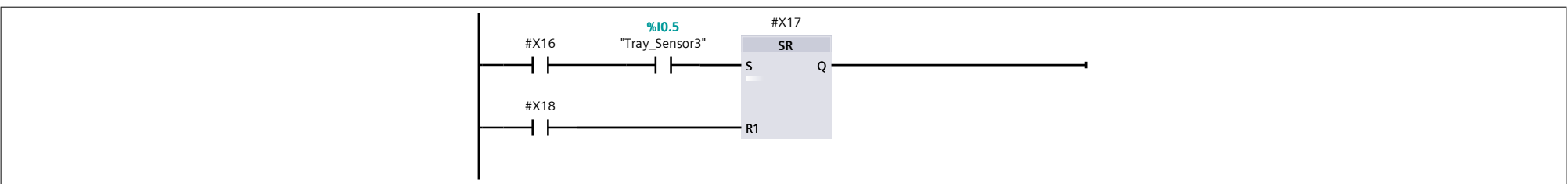
Network 9:
