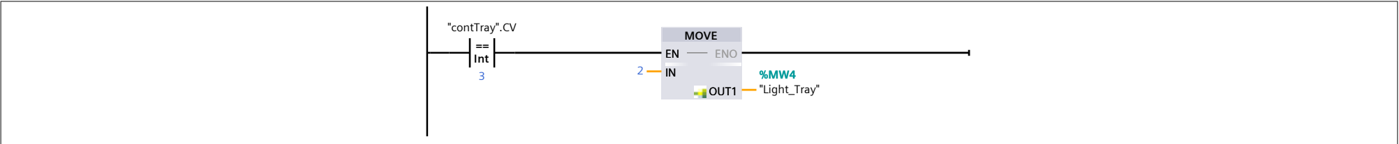
Network 9:
