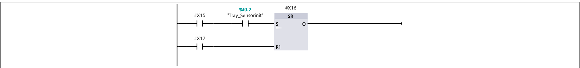
Network 8:
