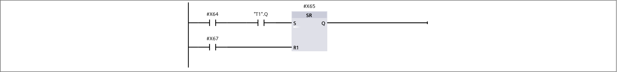
Network 7:
