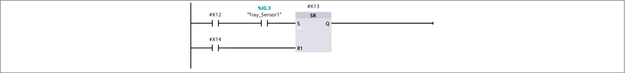
Network 5:
