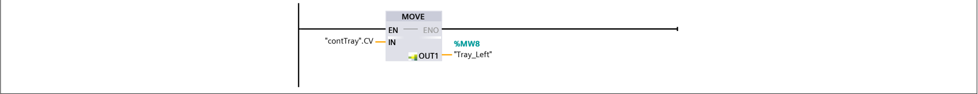
Network 14:
