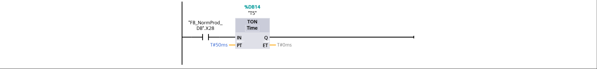
Network 7:
