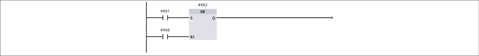
Network 4:
