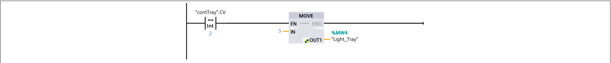
Network 10:
