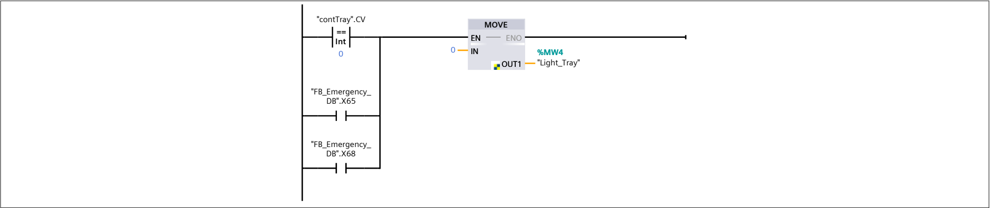
Network 12:
