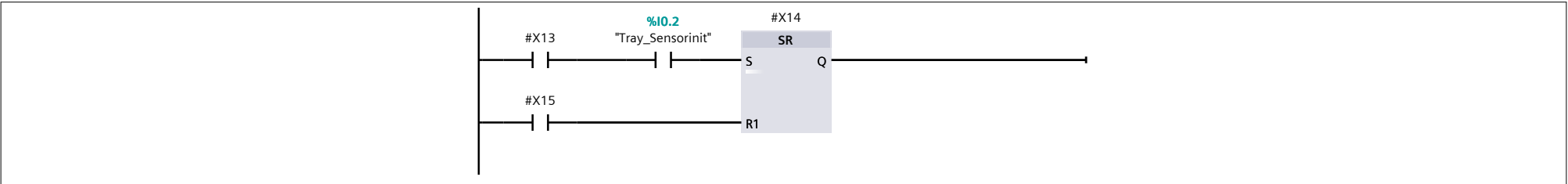
Network 6:
