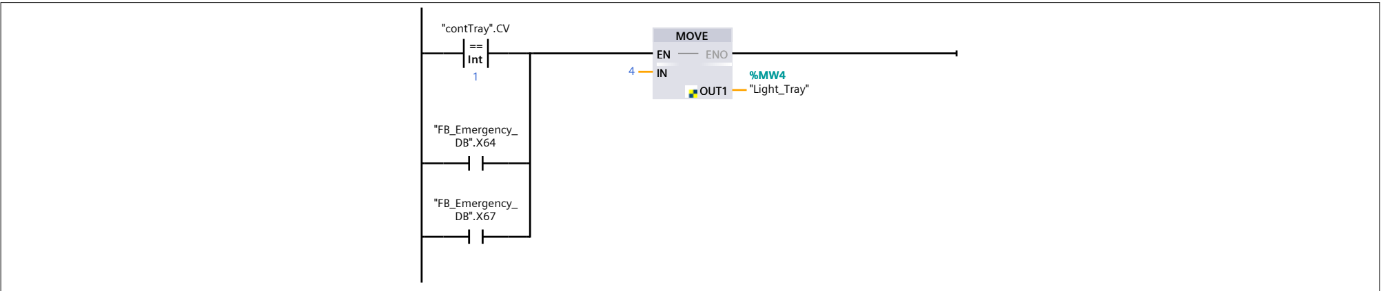
Network 11:
