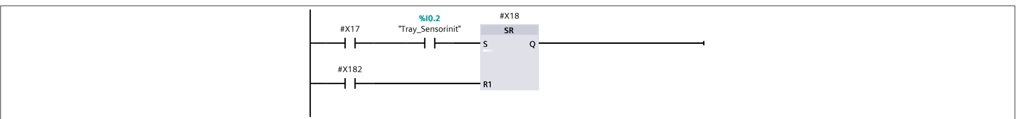
Network 10:
