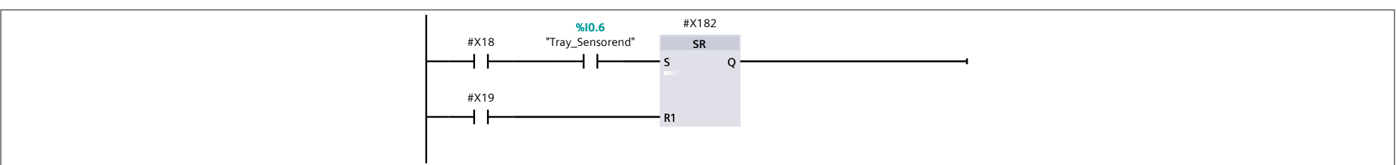
Network 11:
