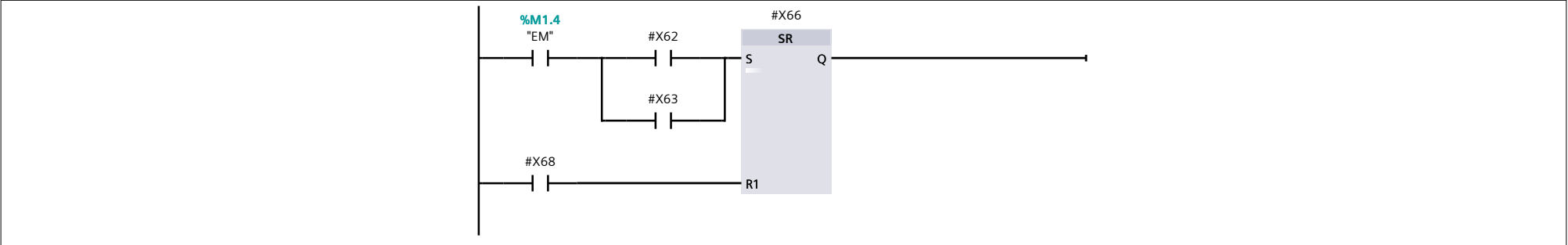
Network 8:
