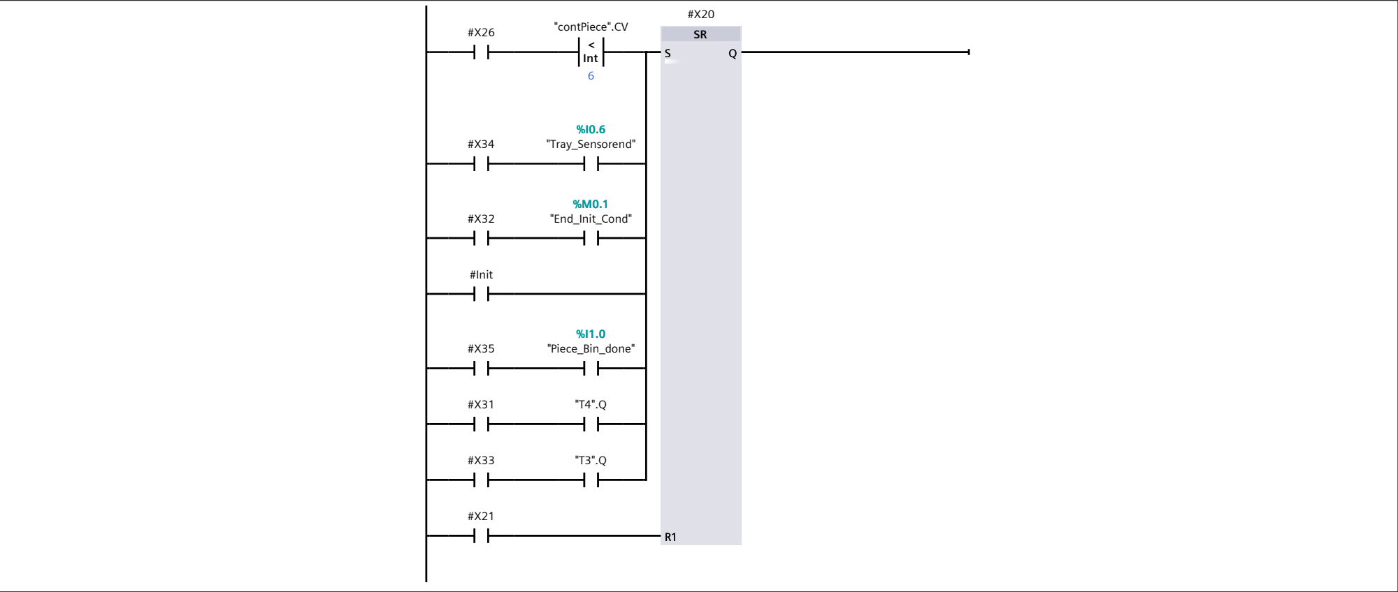
Network 2:
