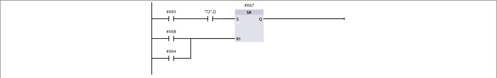
Network 9:
