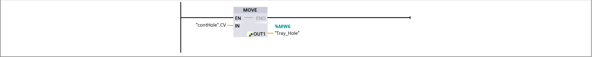
Network 13:
