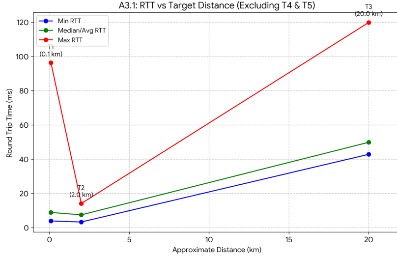
Figure 3.1: Minimum, median/average, and maximum RTT against approximate distance for T1, T2, and T3. T4 is excluded (100% packet loss). T5 is excluded from this plot to preserve the linear distance scale, since its nominal 12,000 km would compress T1–T3 into an unreadable cluster near the origin; T5 is analysed in the text below instead.
