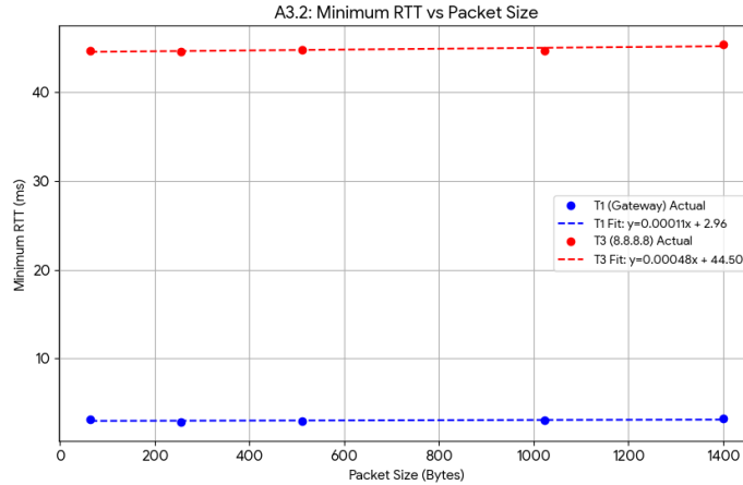
Figure 3.2: Minimum RTT against packet size for T1 and T3, with linear fits.
