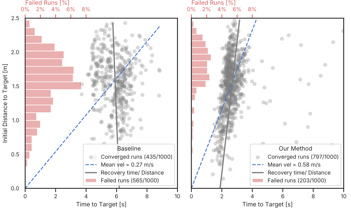
Figure 5.8: Comparison of the learned policy with the baseline method from [16]. We compared the methods on N=1000 runs initialized in harsh conditions. The left plot shows the baseline method. The right plot shows the learned policy. Our method achieves a significantly lower recovery time and failure rate.
