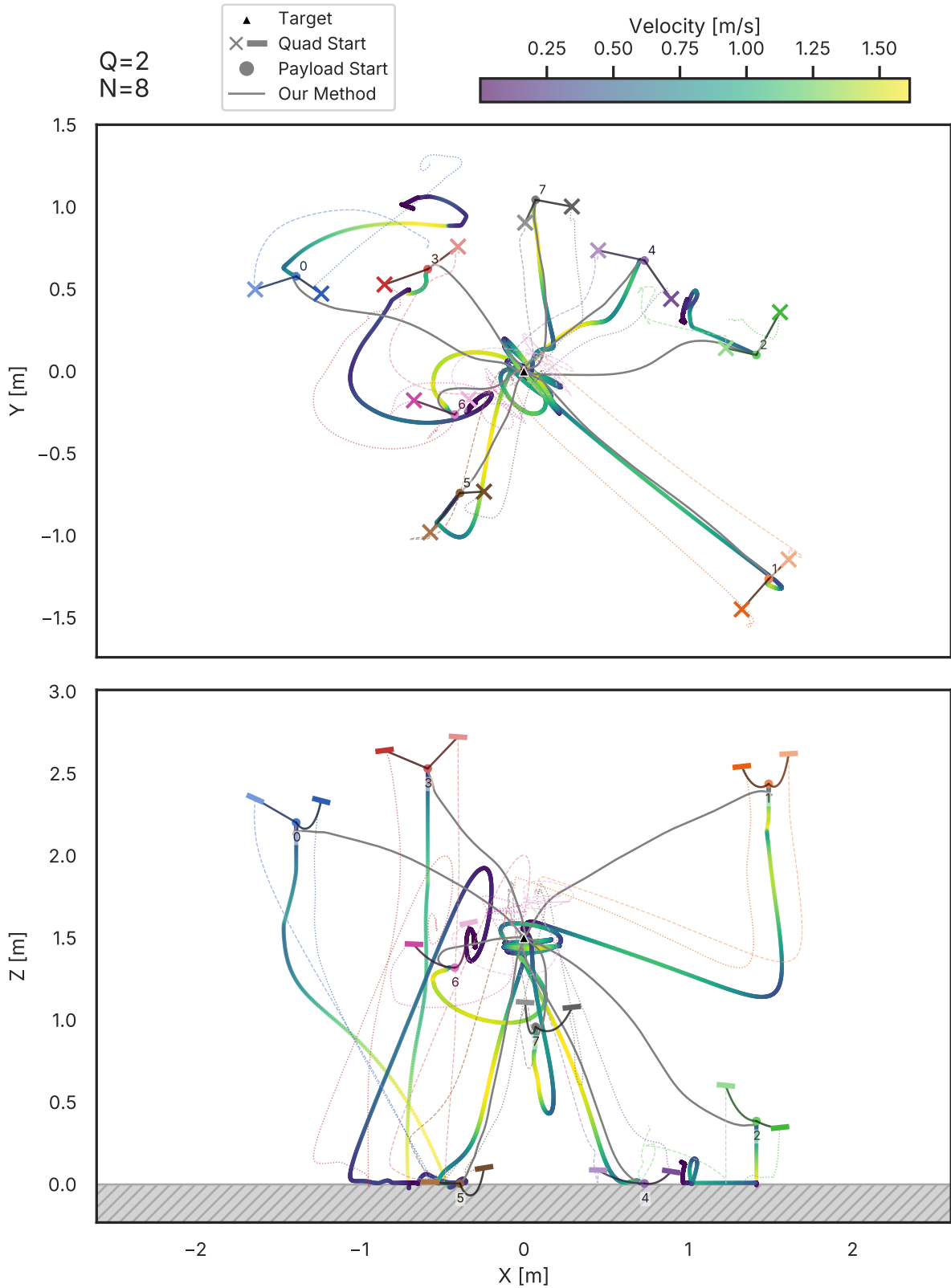
Figure 5.9: Comparison of the learned policy with the baseline method from [16]. Recovery of two quadrotors with payload from harsh conditions. The top plot is a top-down (xy) view, while the bottom one is a side view (xz). The colormapped line shows the baseline method, while the thin gray line shows the learned policy as evaluated before.
