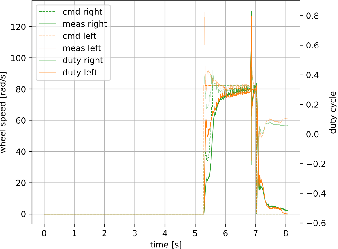
Wheel Speeds
