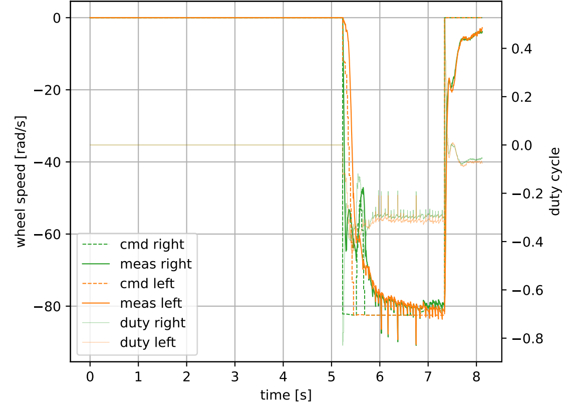
Wheel Speeds
