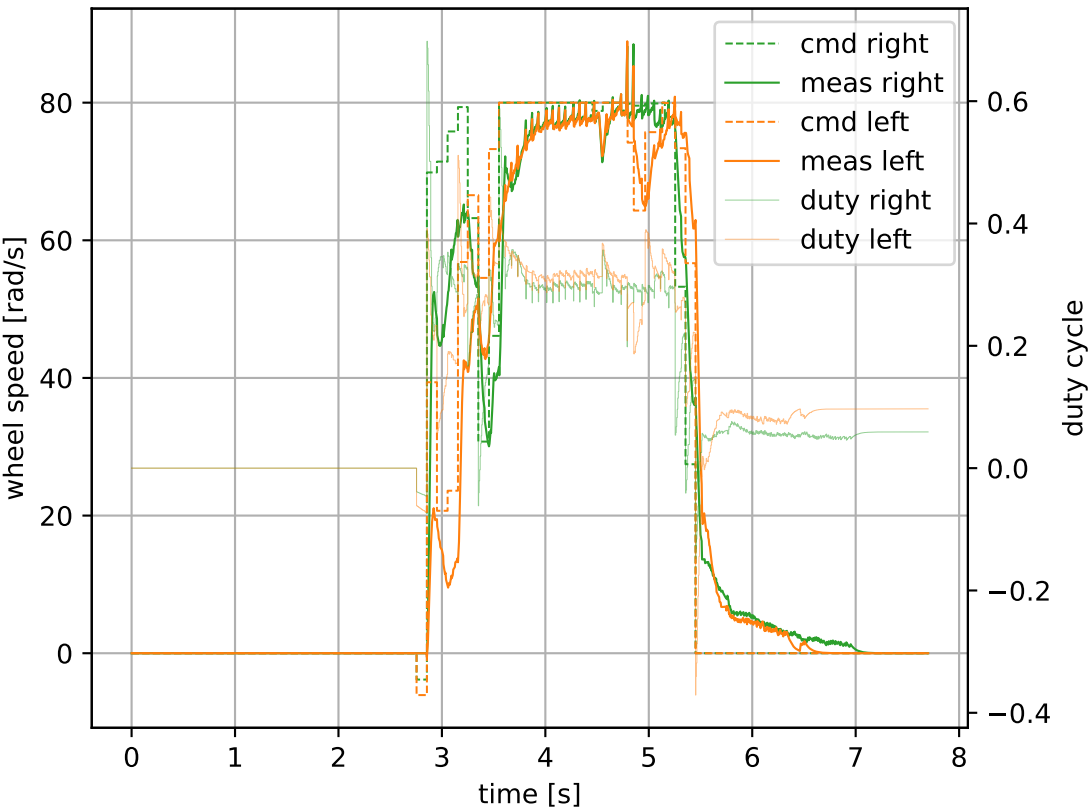
Wheel Speeds
