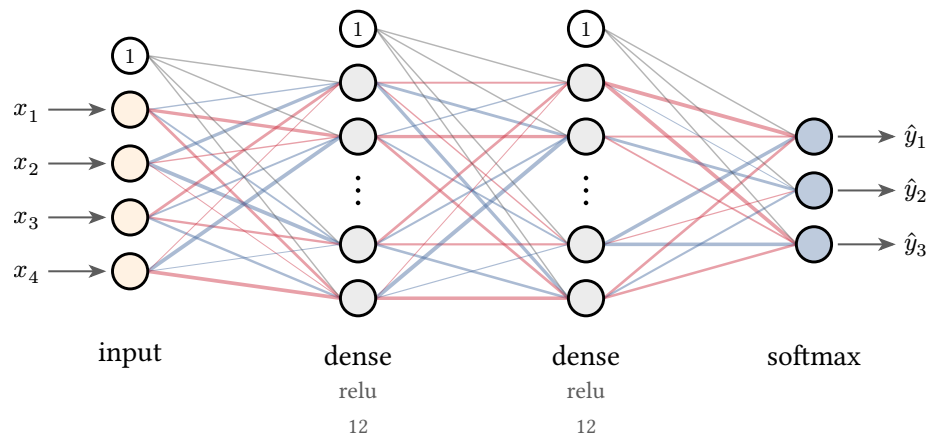
A classifier, weights shown
