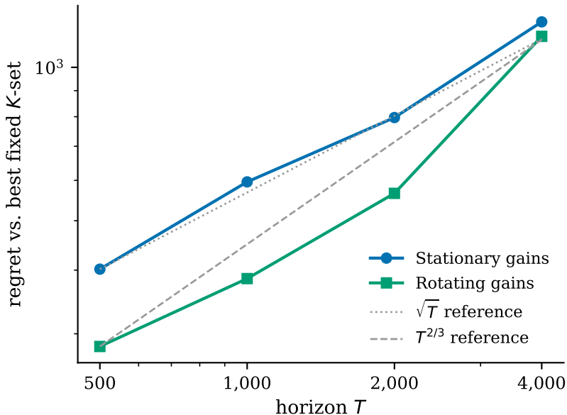
Semi-bandit EXP3.M ( W = 50, K = 5 )
