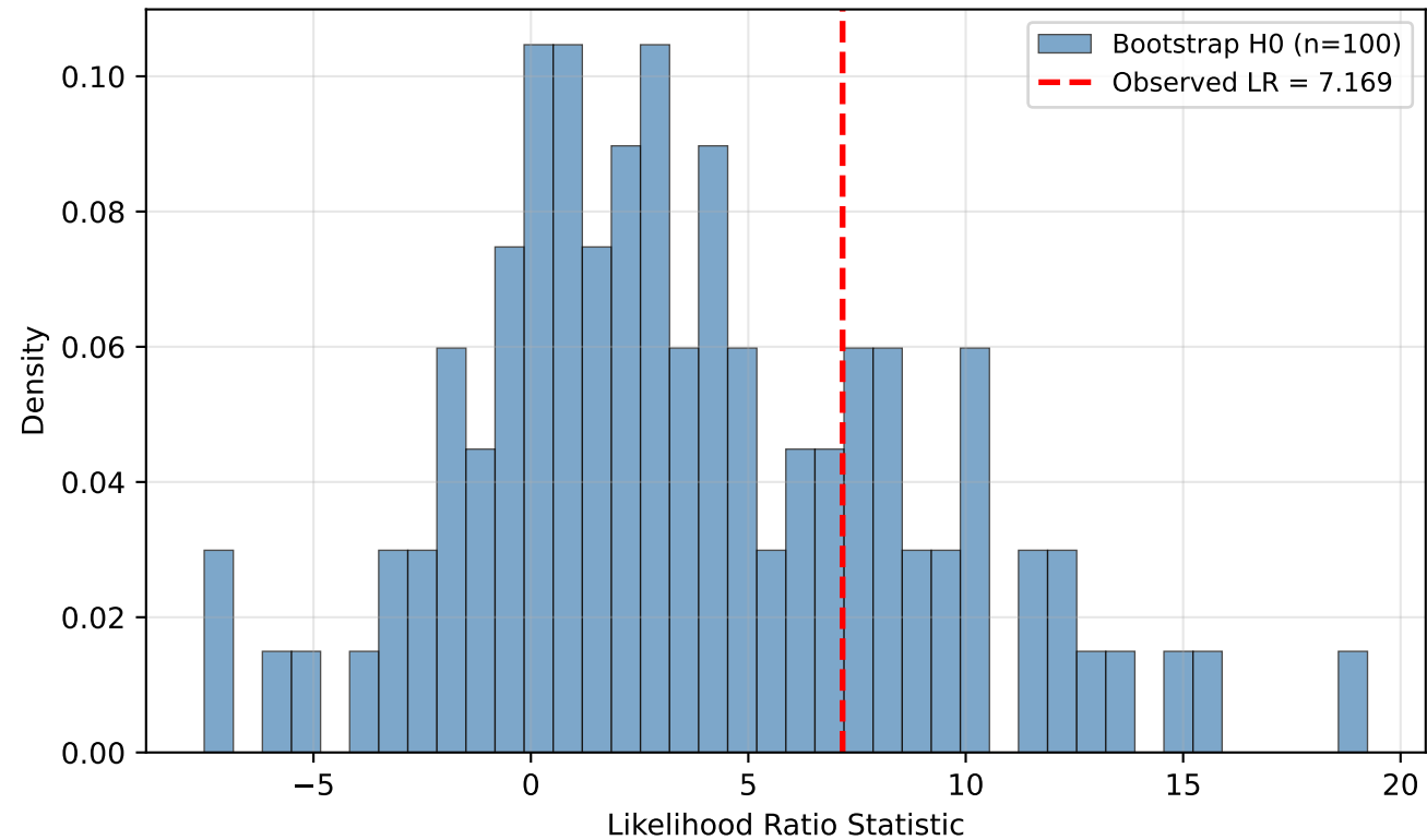
Test C: Parametric Bootstrap [VIDE] ( p=0.250 )
