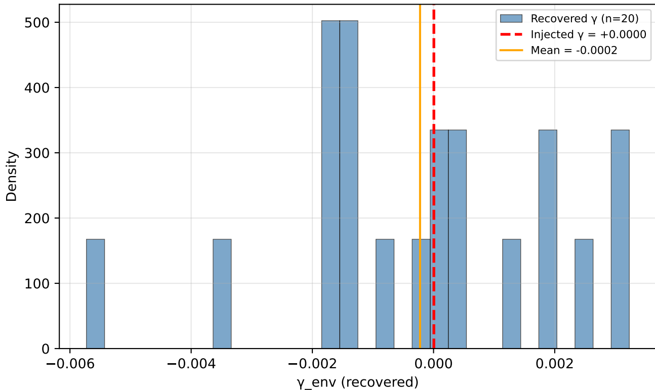
Test E: SGC Recovery [VOIDFINDER] 0.5x (bias=-0.0002)
