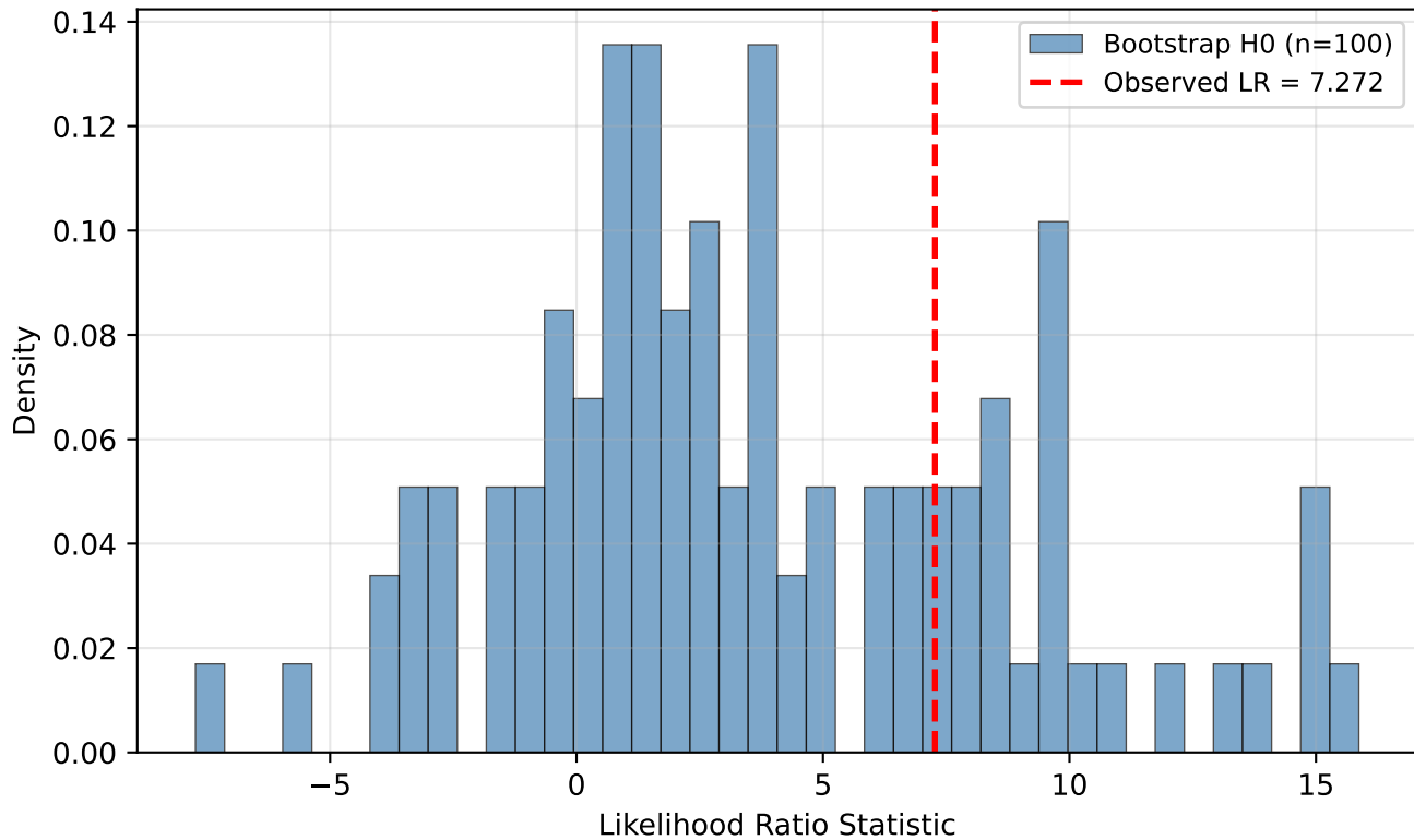
Test C: Parametric Bootstrap [VOIDFINDER] ( p=0.250 )
