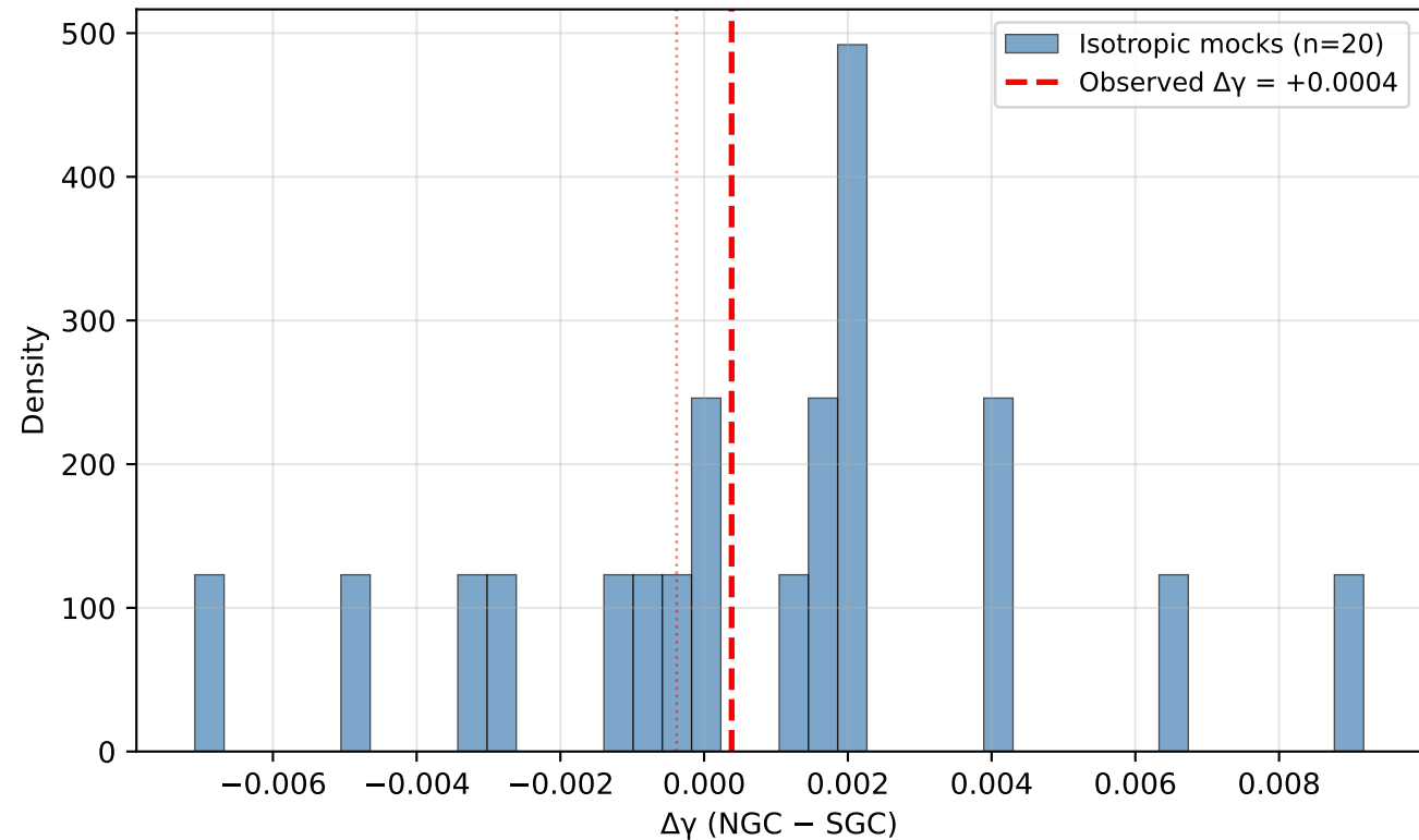
Test D: Geometry Mocks [VIDE] ( p=0.900 )
