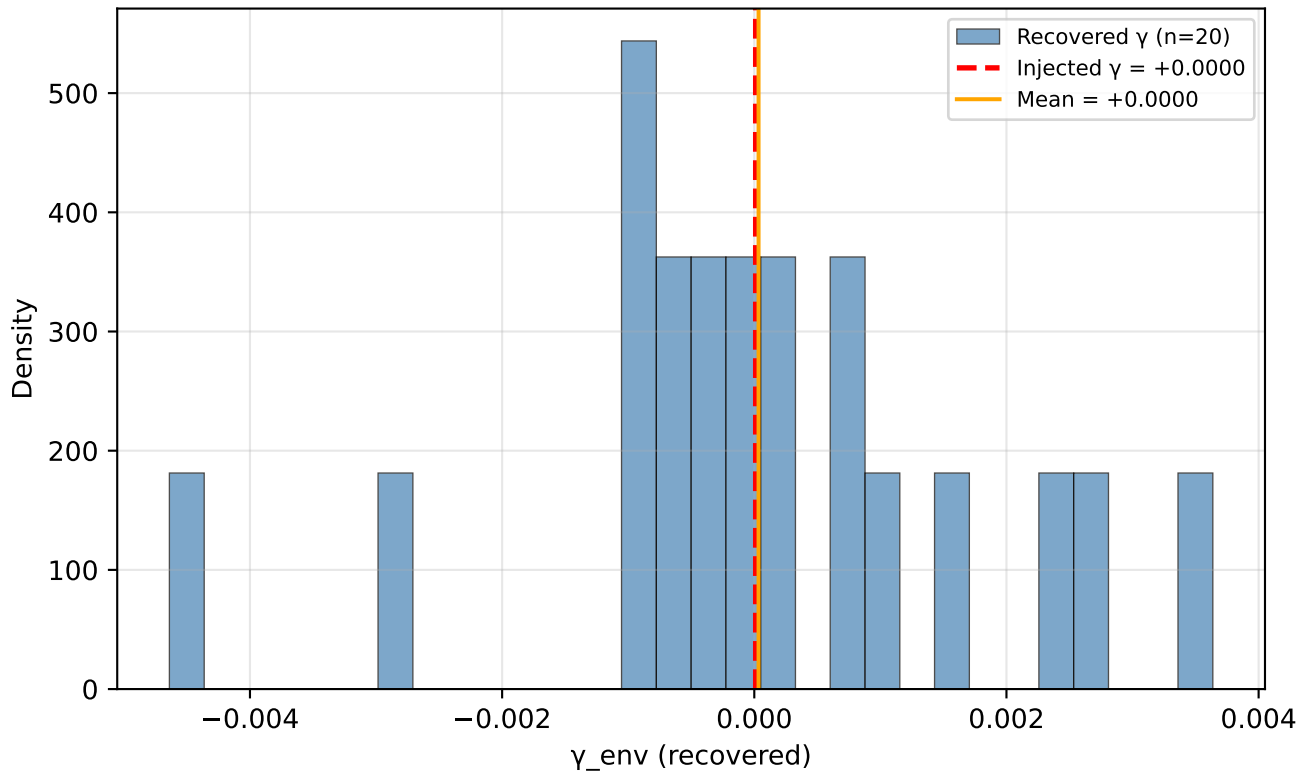
Test E: SGC Recovery [VOIDFINDER] 1.0x (bias=+0.0000)
