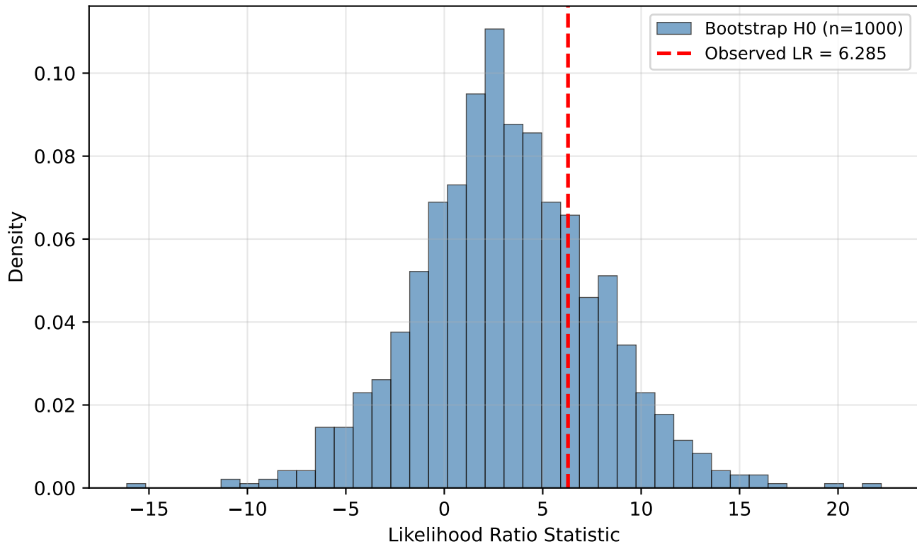
Test C: Parametric Bootstrap [REVOLVER] ( p=0.243 )
