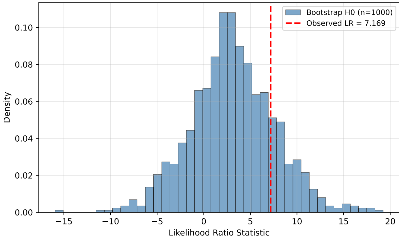
Test C: Parametric Bootstrap [VIDE] ( p=0.179 )
