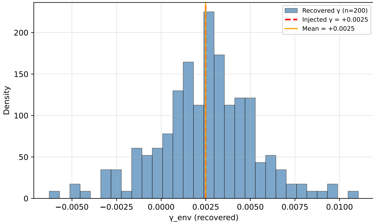
Test E: SGC Recovery [REVOLVER] 0.5x (bias=-0.0000)
