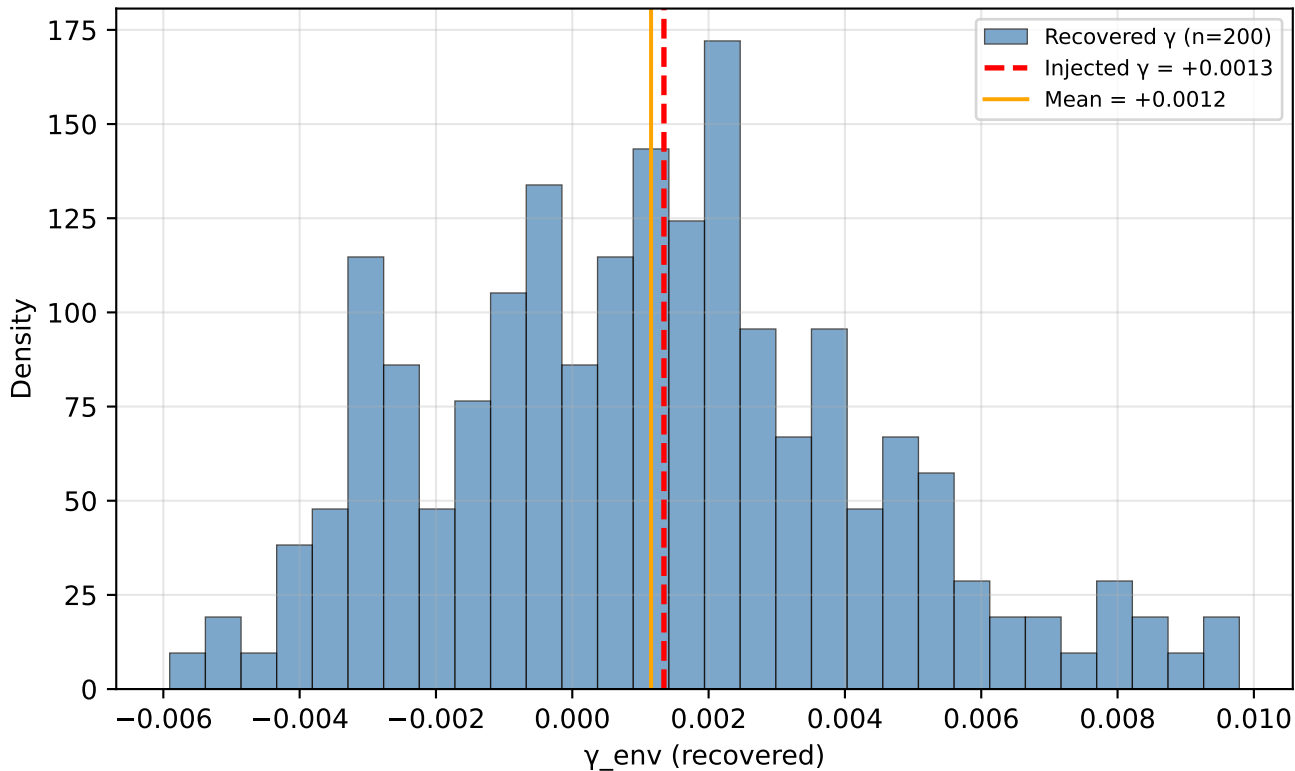
Test E: SGC Recovery [VIDE] 0.5x (bias=-0.0002)
