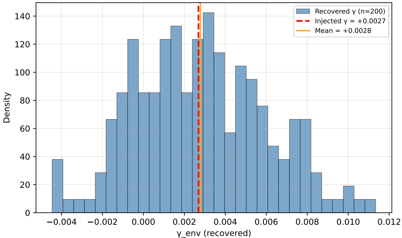
Test E: SGC Recovery [VIDE] 1.0x (bias=+0.0001)
