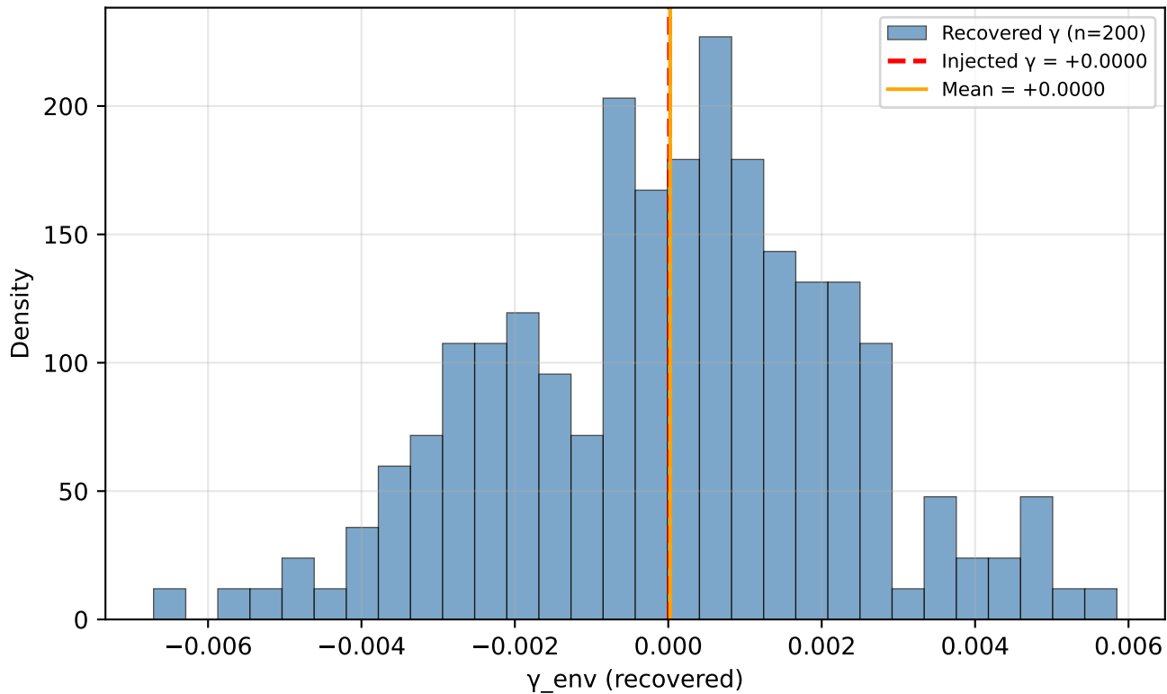
Test E: SGC Recovery [VOIDFINDER] 1.5x (bias=+0.0000)
