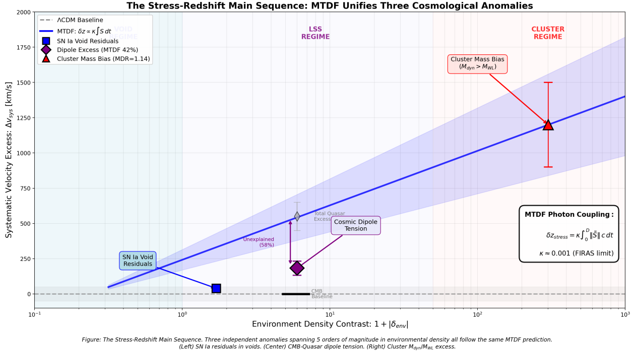
Figure A.1. The stress-redshift main sequence synthesis plot (generated by mtdf_synthesis_plot.py ).
