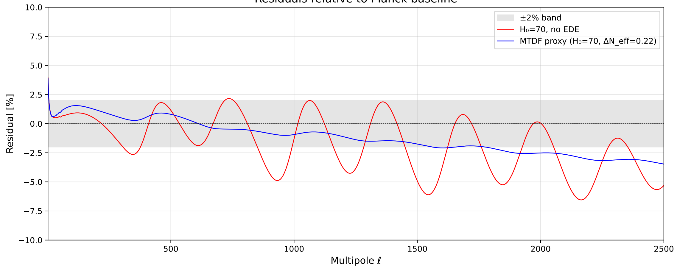
Residuals relative to Planck baseline
