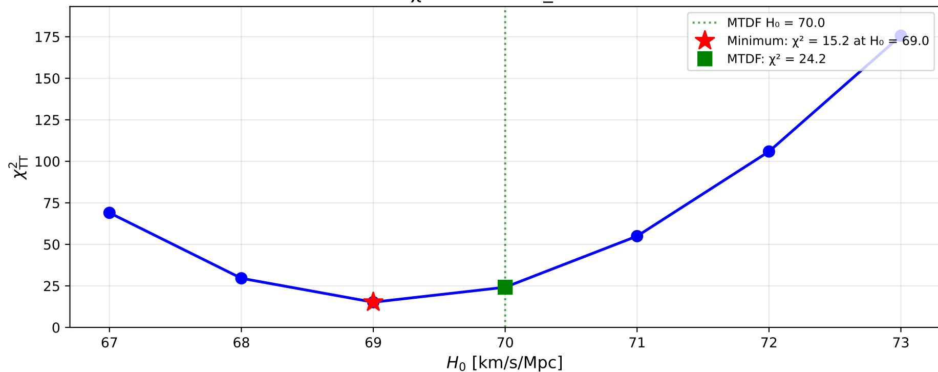
CMB \chi^2 vs H_0 at \Delta N_{\text{eff}} = 0.22
