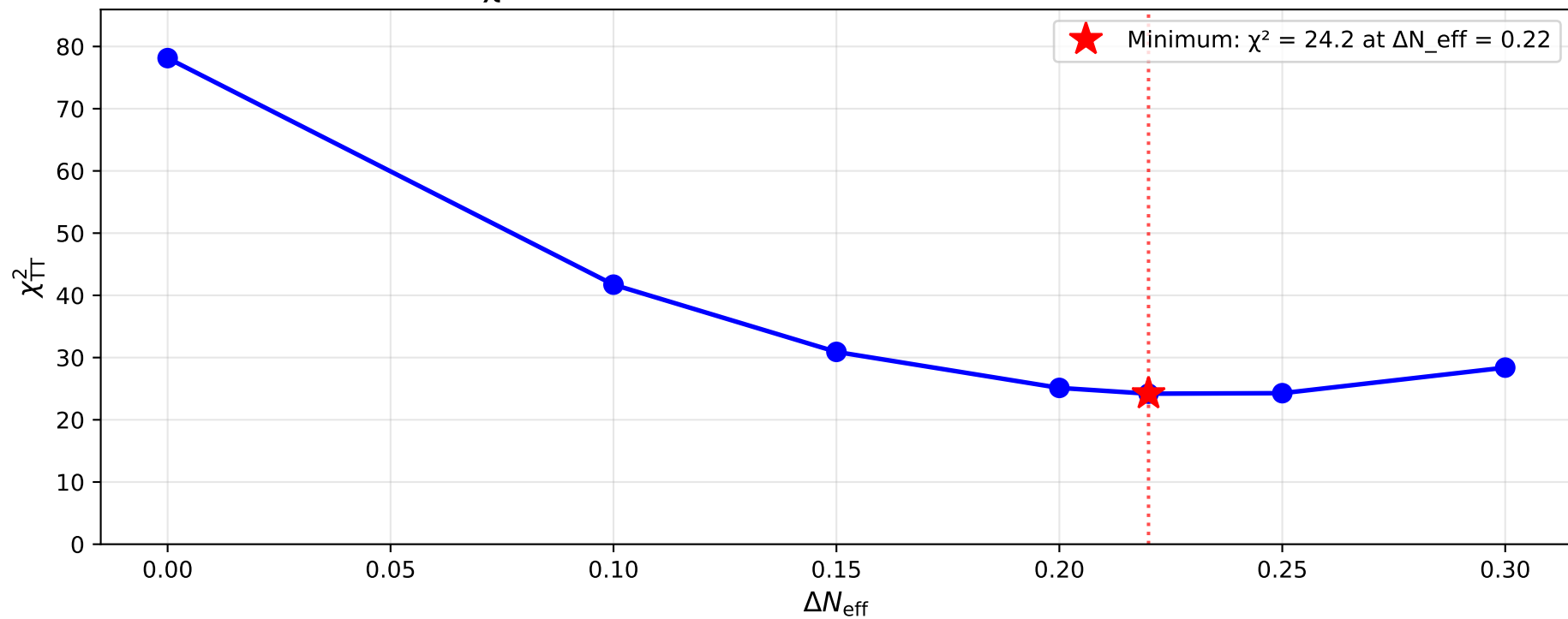
CMB \chi^2 vs Extra Radiation (relative to Planck baseline)
