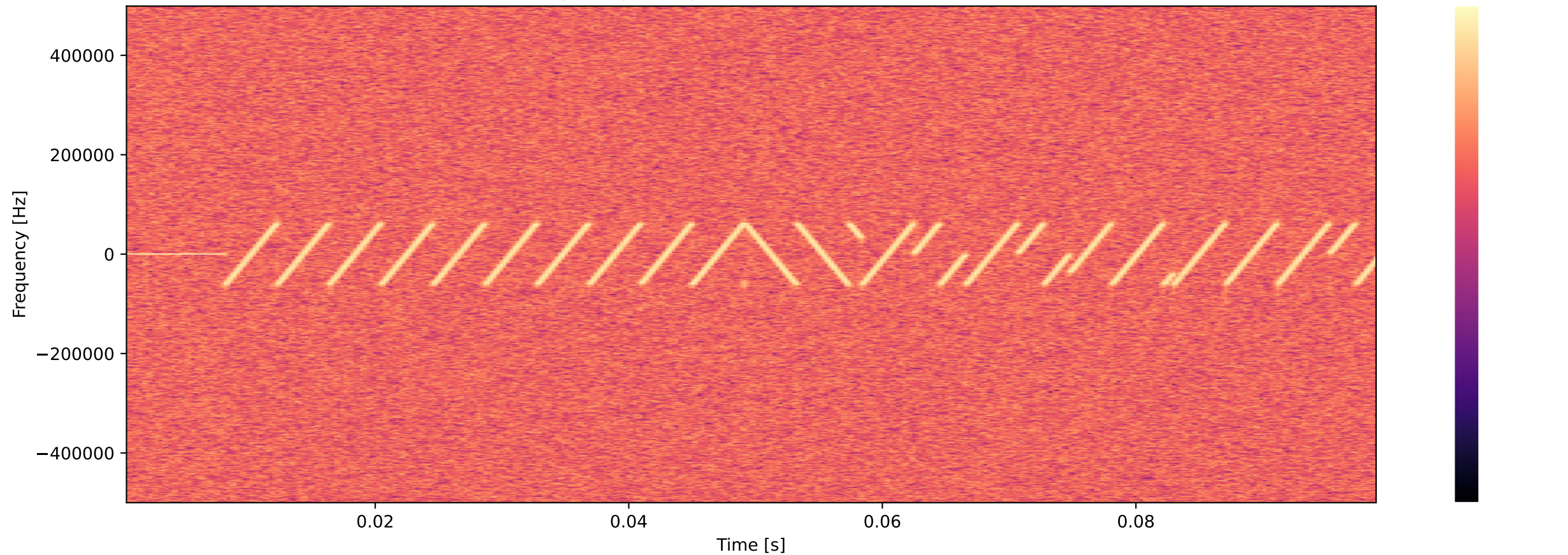
LoRa Signal Spectrogram (After CFO/STO Correction)
