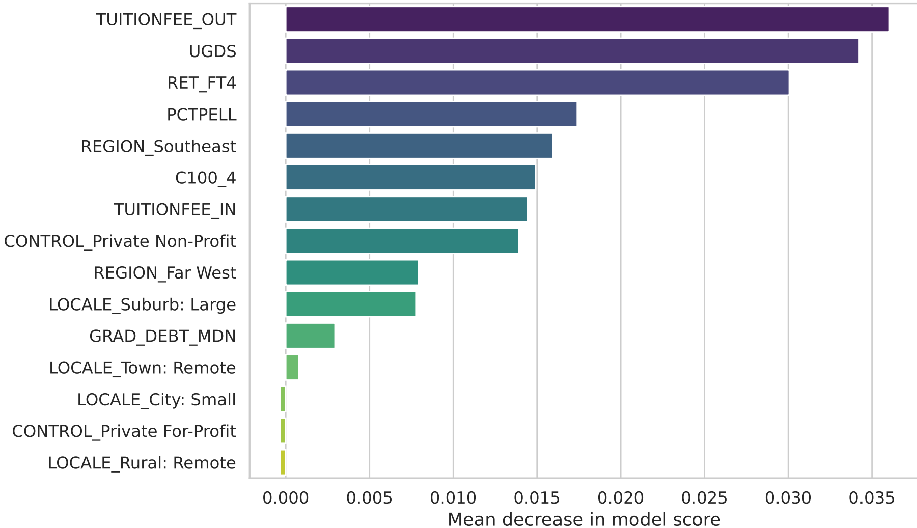
Top 15 Features by Permutation Importance (Random Forest)
