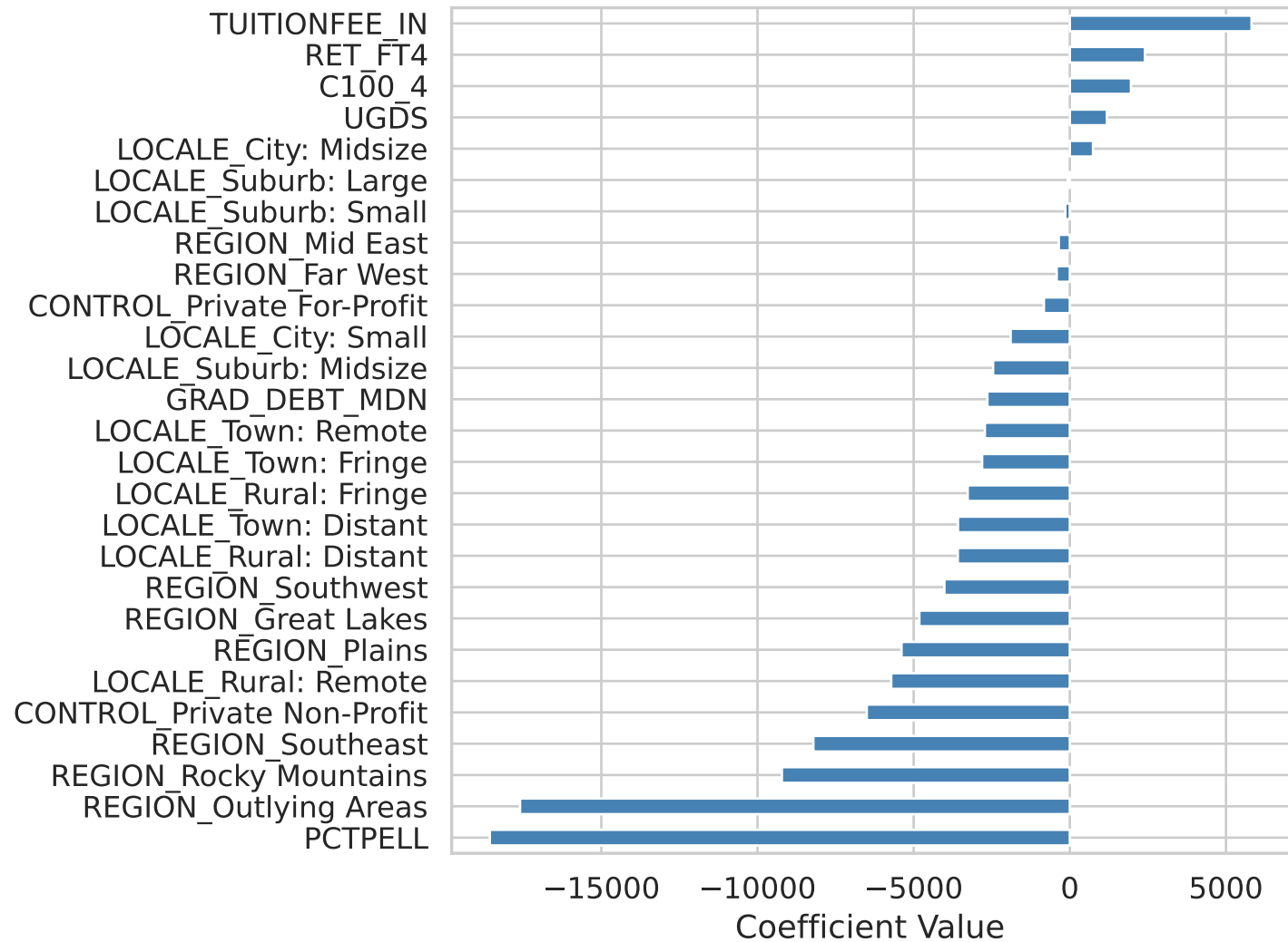
OLS Regression Coefficients
