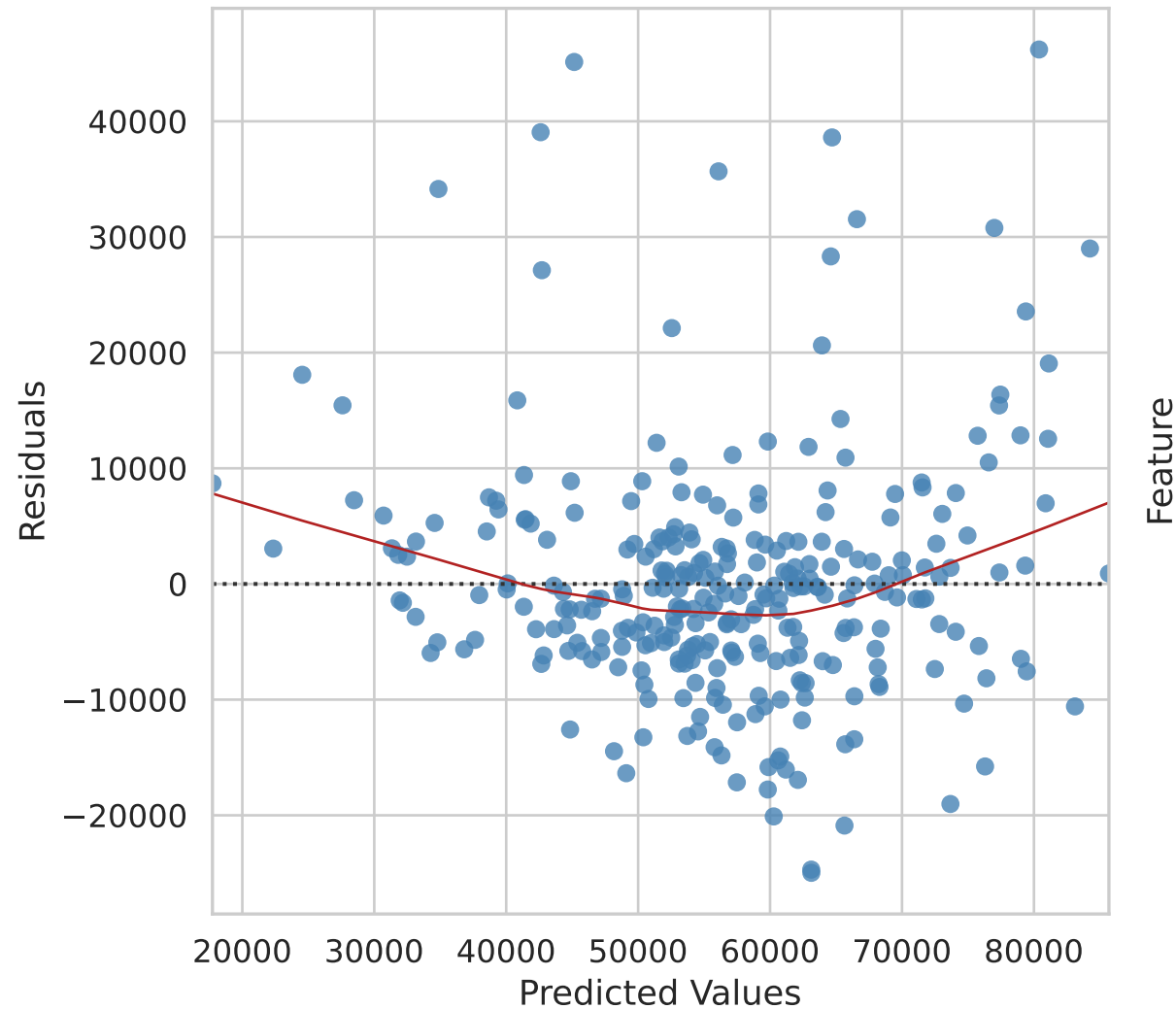
Residual Plot for OLS Regression
