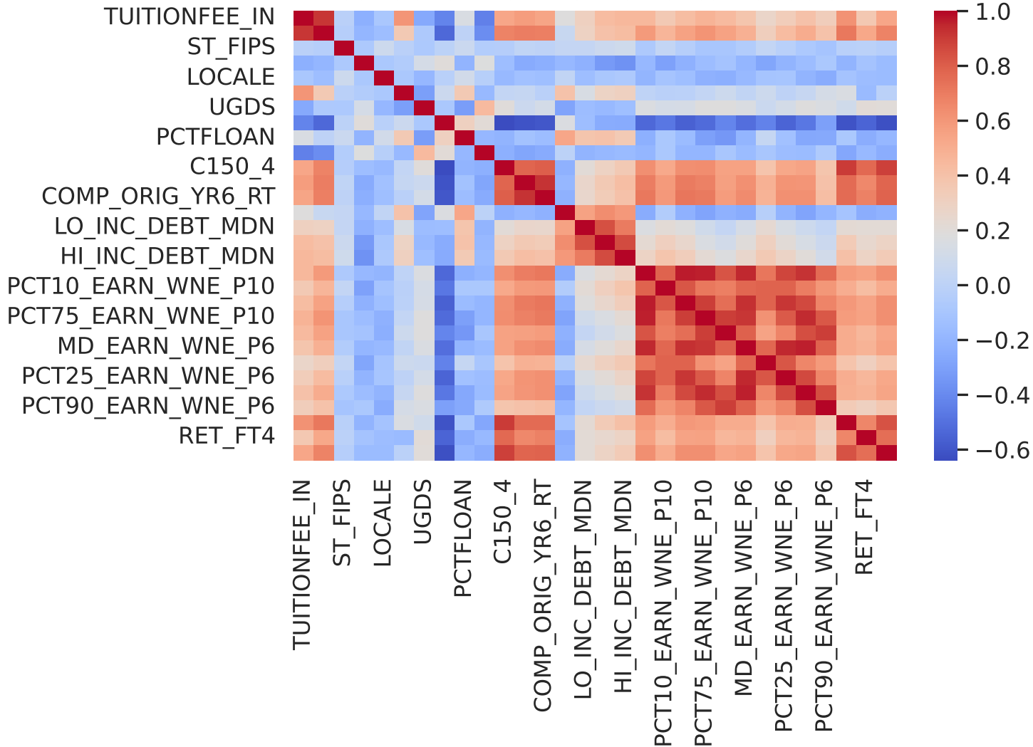
Correlation Matrix of Numerical Variables
