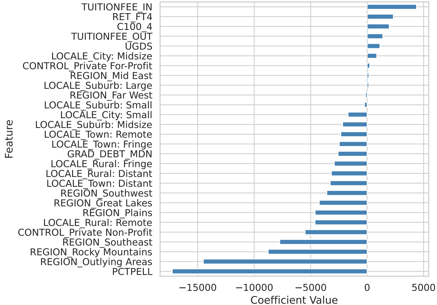
Ridge Regression Coefficients
