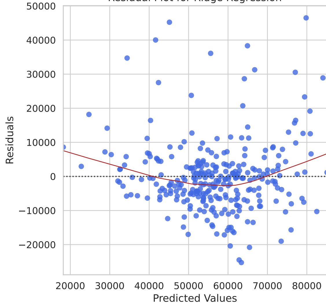
Residual Plot for Ridge Regression
