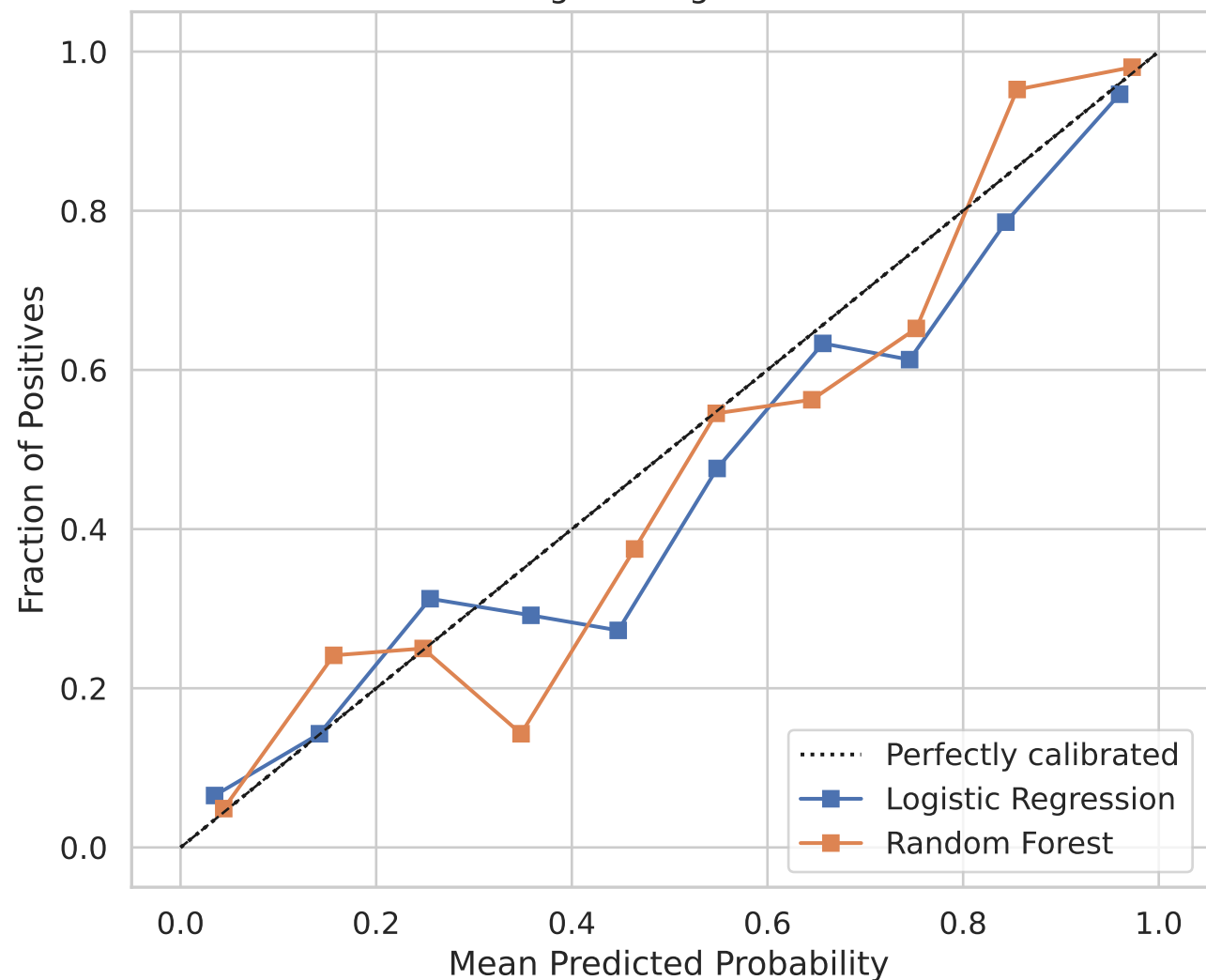
Calibration Curve: Logistic Regression vs Random Forest
