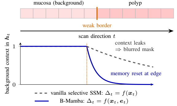
Fig. 1. The problem B-Mamba addresses (conceptual sketch, not measured data). A selective SSM reads image tokens one after another and keeps a running memory h_t . How fast it forgets is set by the step size \Delta_t . In existing vision Mamba models \Delta_t depends only on the local appearance x_t ; at a weak border the appearance barely changes, so background context keeps flowing into the polyp region. B-Mamba also feeds an explicit boundary token e_t into \Delta_t , B_t and C_t , so the scan can learn to reset its memory exactly at the edge. Measured step-size maps are shown in Fig. 4.
