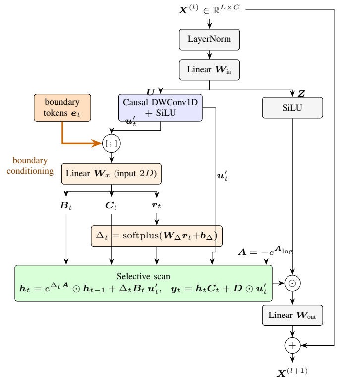
Fig. 3. The Boundary-Conditioned SSM block. Orange parts are new compared with a standard Mamba block: the boundary token \mathbf{e}_t is concatenated with the visual token \mathbf{u}'_t before the projection that produces the step size \Delta_t and the matrices \mathbf{B}_t, \mathbf{C}_t . Everything else, including the linear-time scan, is unchanged.
