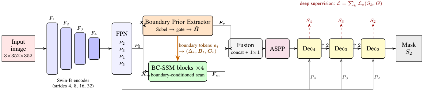
Fig. 2. Overview of B-Mamba. A Swin-B encoder and a feature pyramid network (FPN) produce multi-scale features P_2 – P_5 . At the coarsest level, two parallel branches process P_5 : the Boundary Prior Extractor (BPE) computes a Sobel prior and a boundary-gated texture feature, and the BC-SSM branch models global context with a selective scan whose parameters are conditioned on the boundary tokens produced by the BPE (orange arrow). The two outputs are fused and decoded by an ASPP module and a three-stage progressive decoder with lateral FPN connections. Side outputs S_4, S_3, S_2 are supervised during training; only S_2 is used at test time.
