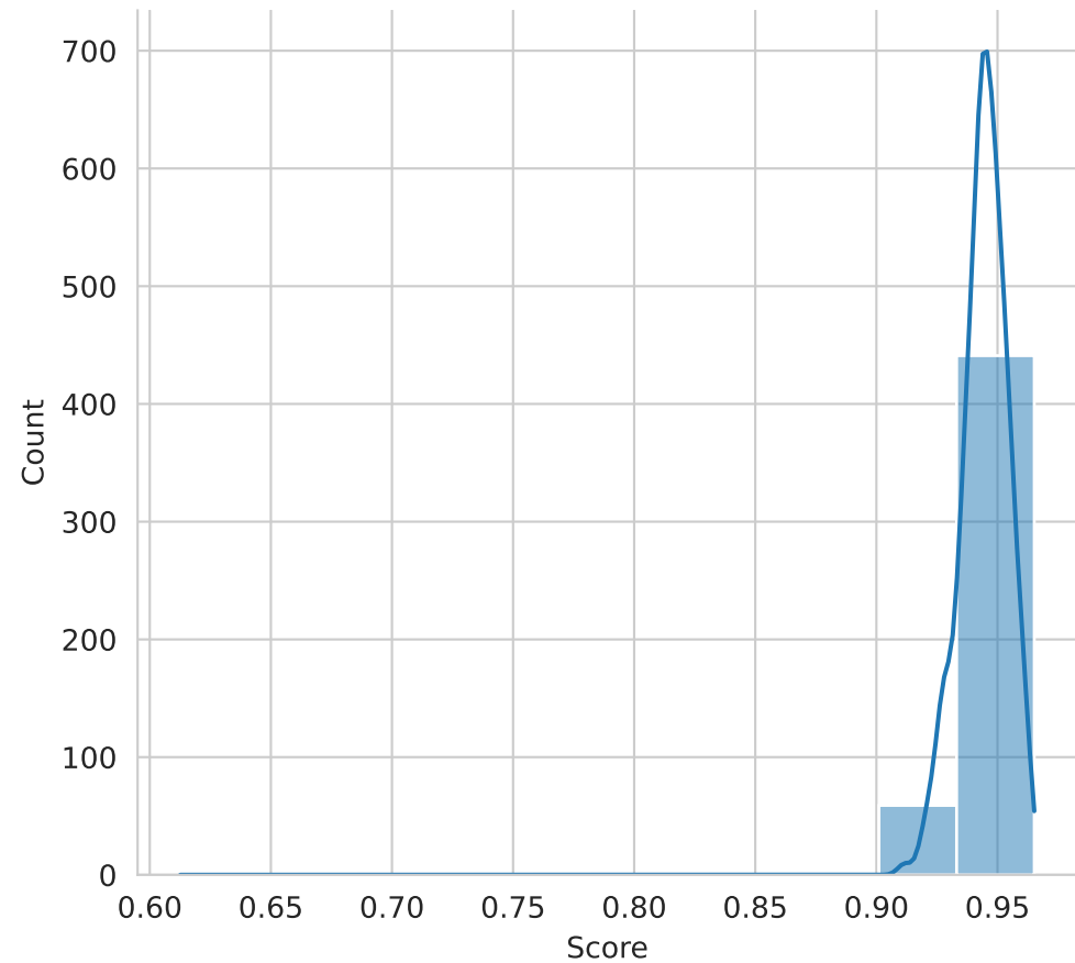
Performance = f1_score(0)
