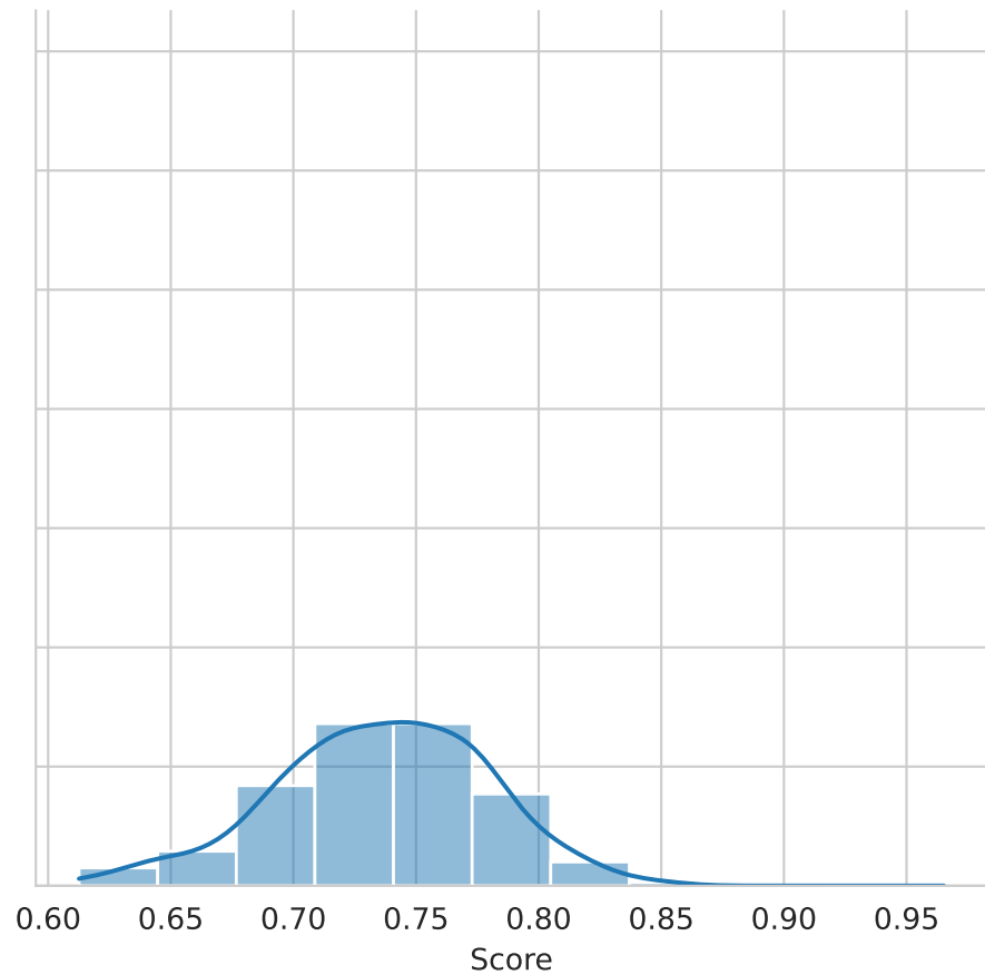
Performance = f1_score(1)
