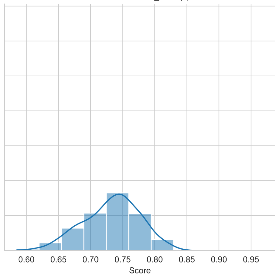
Performance = f1_score(1)
