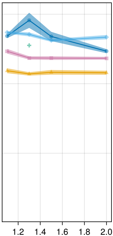
search-cost
