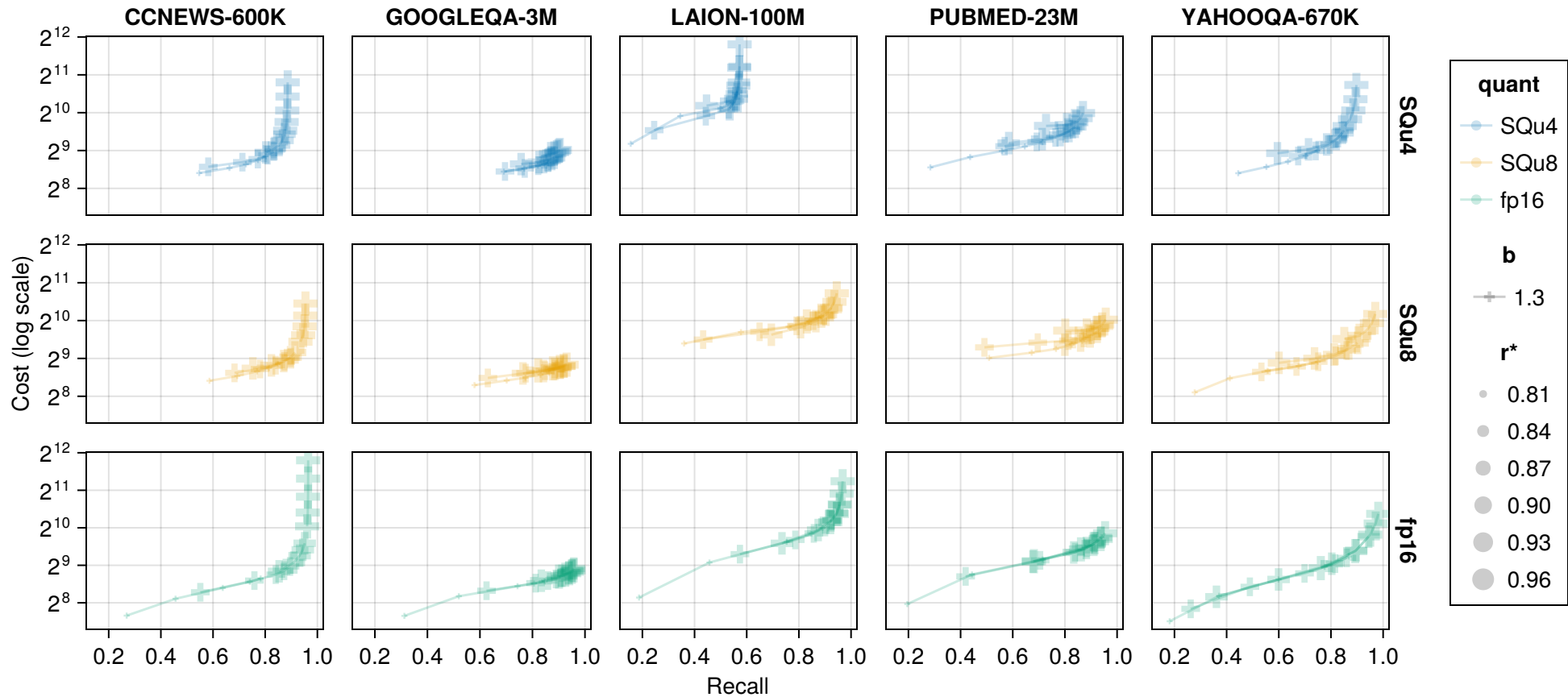
Recall vs Cost per Quant (b=1.3)
