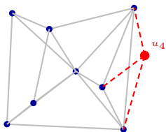
Ins. u_4
