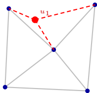
Ins. u_1
