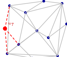
Ins. u_7
