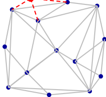
Ins. u_9
