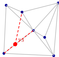
Ins. u_3
