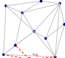
Ins. u_6
