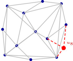
Ins. u_8
