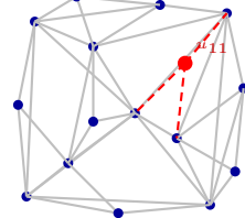
Ins. u_{11}
