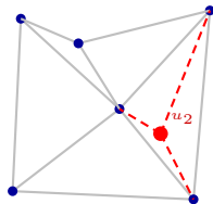
Ins. u_2
