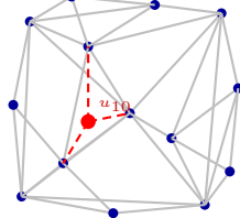
Ins. u_{10}
