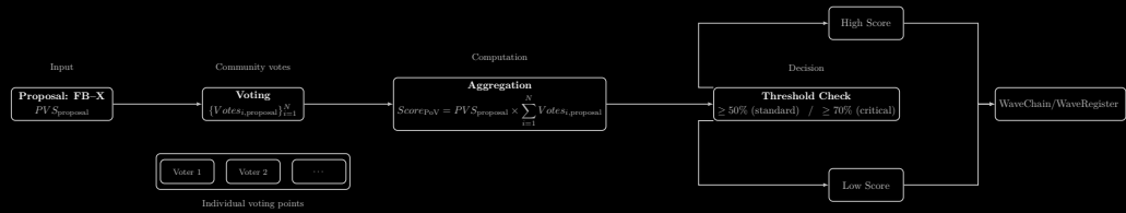
Proof-of-Value (PoV) voting, aggregation, and threshold workflow.
