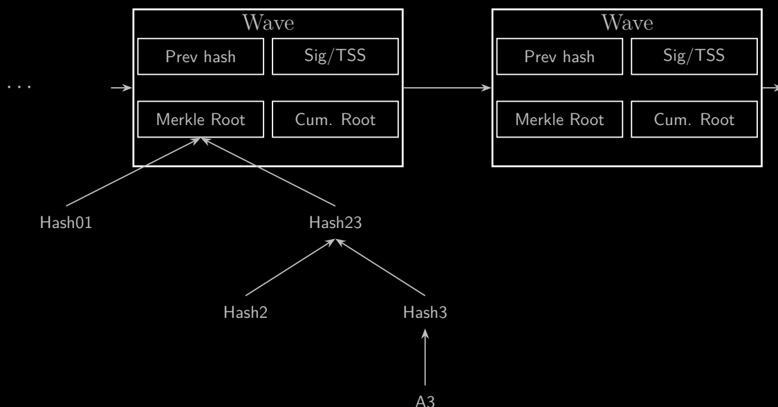
Internal structure of a Wave block and Merkle Root of artifacts.
