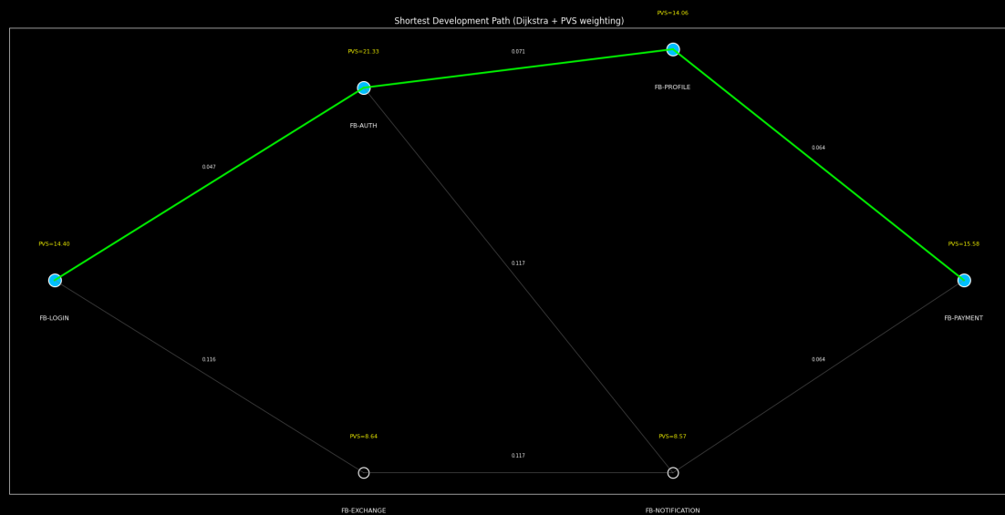
Example Shortest Development Path (Dijkstra).
