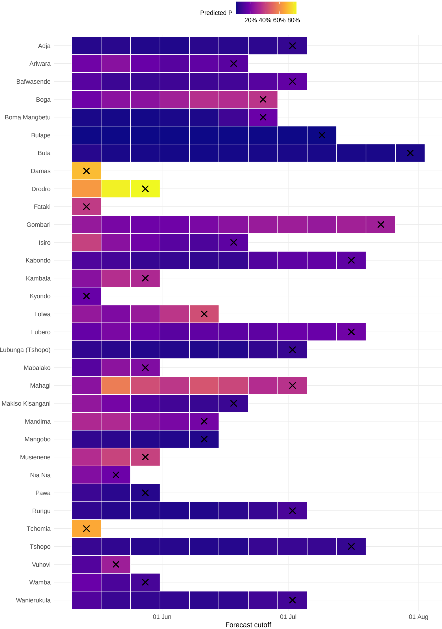
LFO: predicted invasion risk vs realised invasions (Bayes-M17-geo, h=1w) Rows = zones that were invaded; . = the fold at which the invasion occurred
