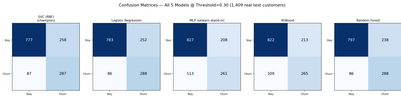
Figure 7: Confusion matrices for all five models at threshold 0.30 on 1,409 real test customers.
