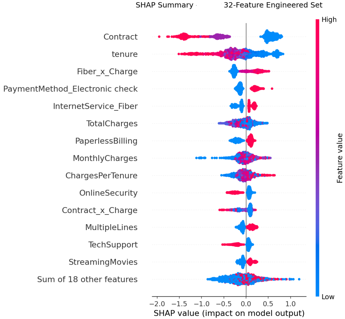
Figure 8: SHAP summary for the 32-feature engineered set. The local image identifies the displayed explainer as XGBoost; it is model-behaviour evidence, not intervention causality.
