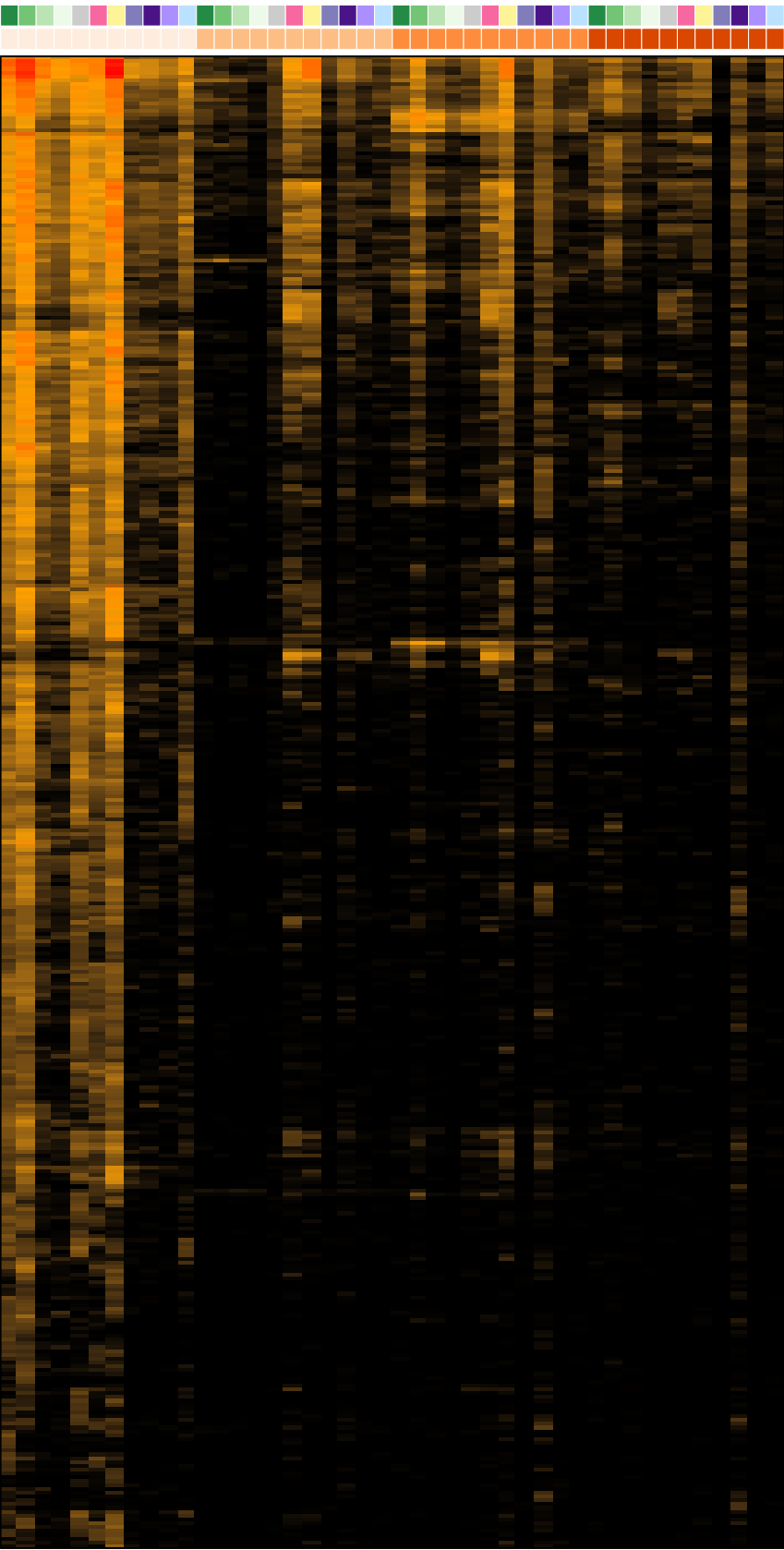
SCPA_GOBP_max_q-val_1
