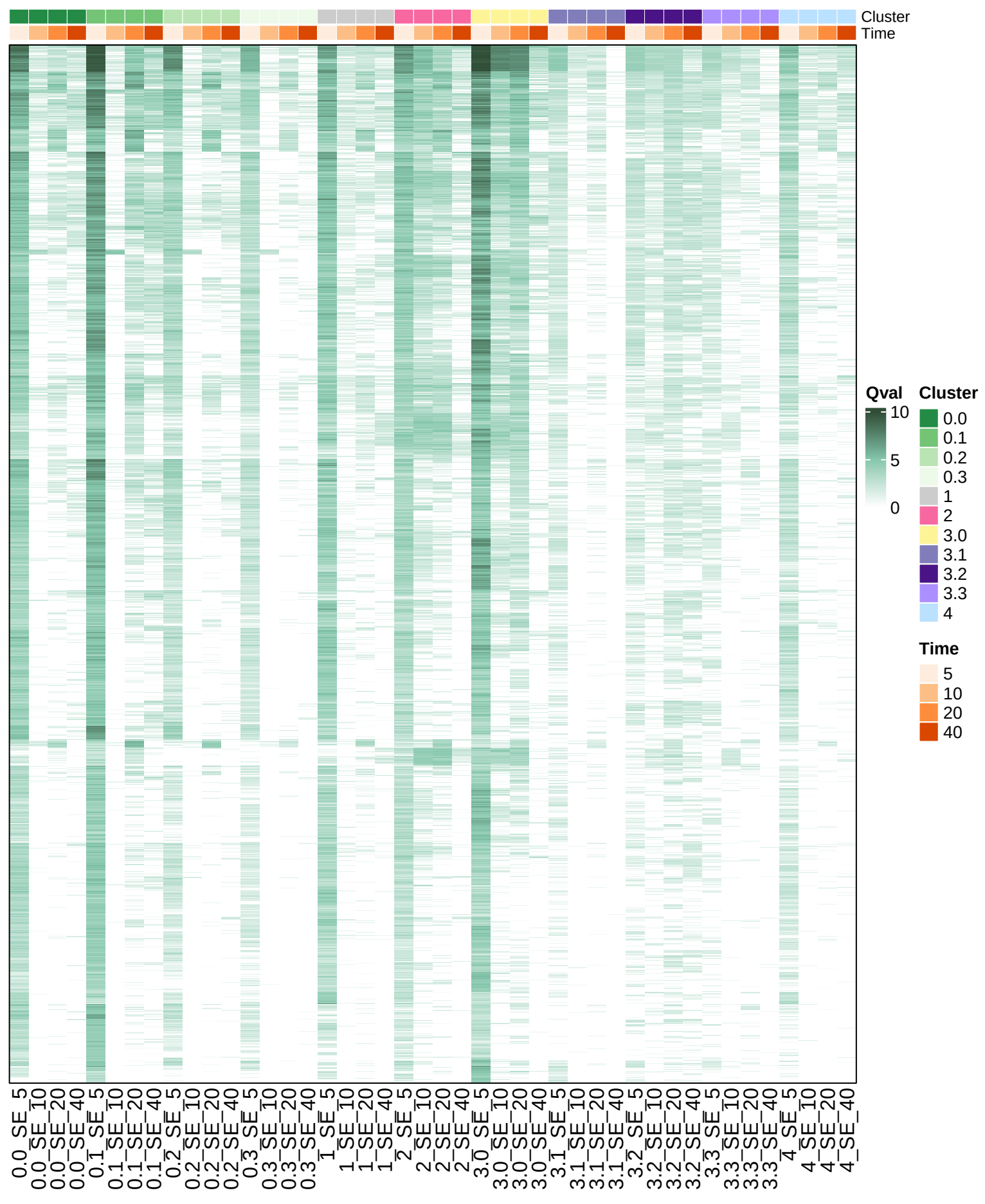
SCPA_GOBP_max_q-val_4
