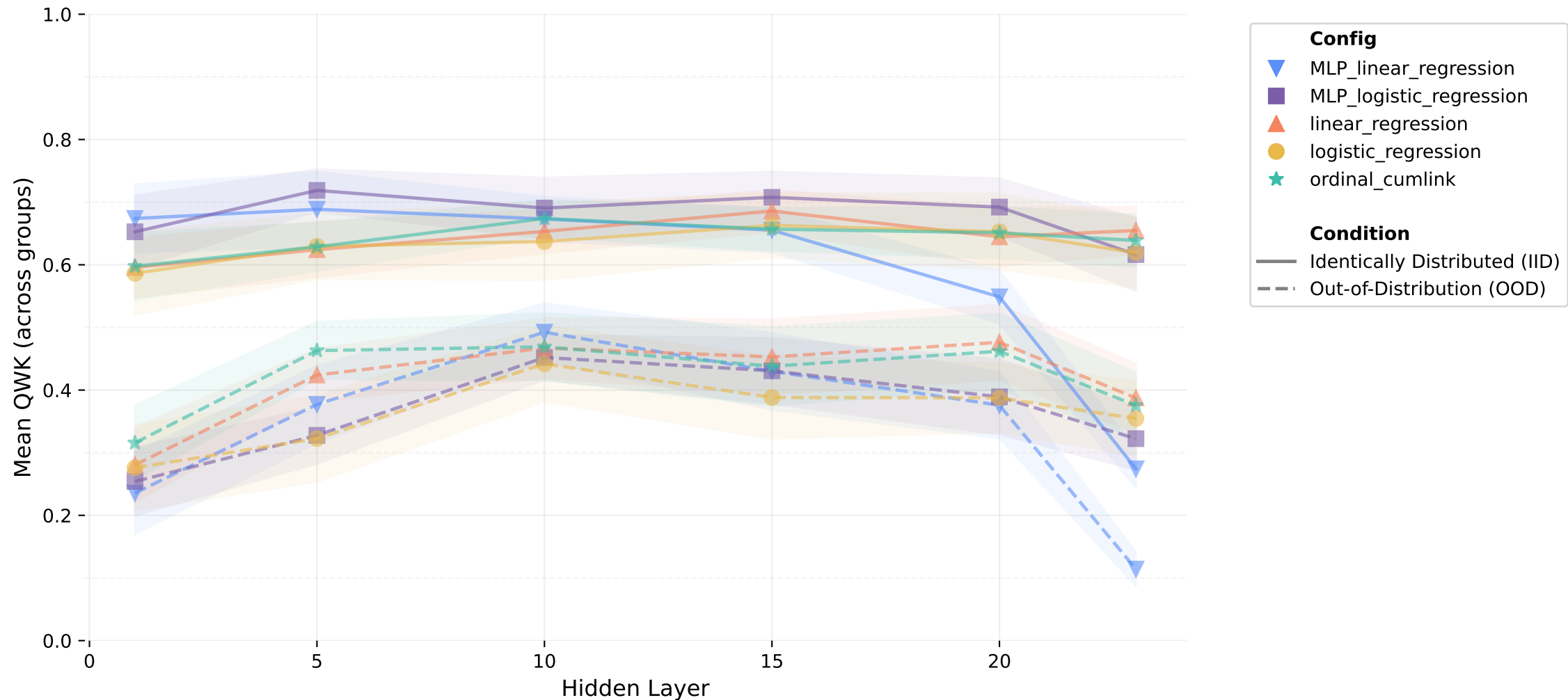
QWK by layer — embeddinggemma-300M — all configs color/marker = config | solid = IID, dashed = OOD | black = XGB surface baseline
