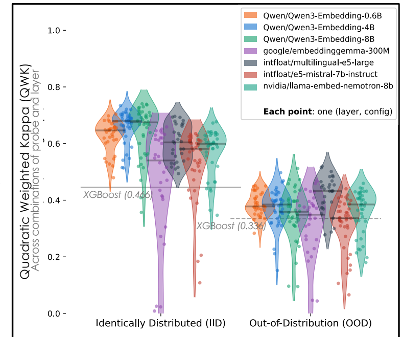
Violin plot showing performance distribution of each trained model.
