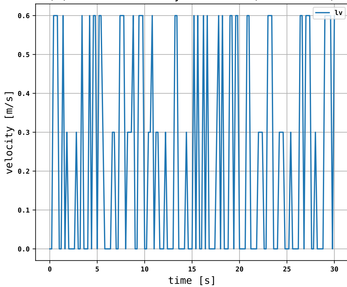
(3) Linear velocity commands (d-modelFMU)
