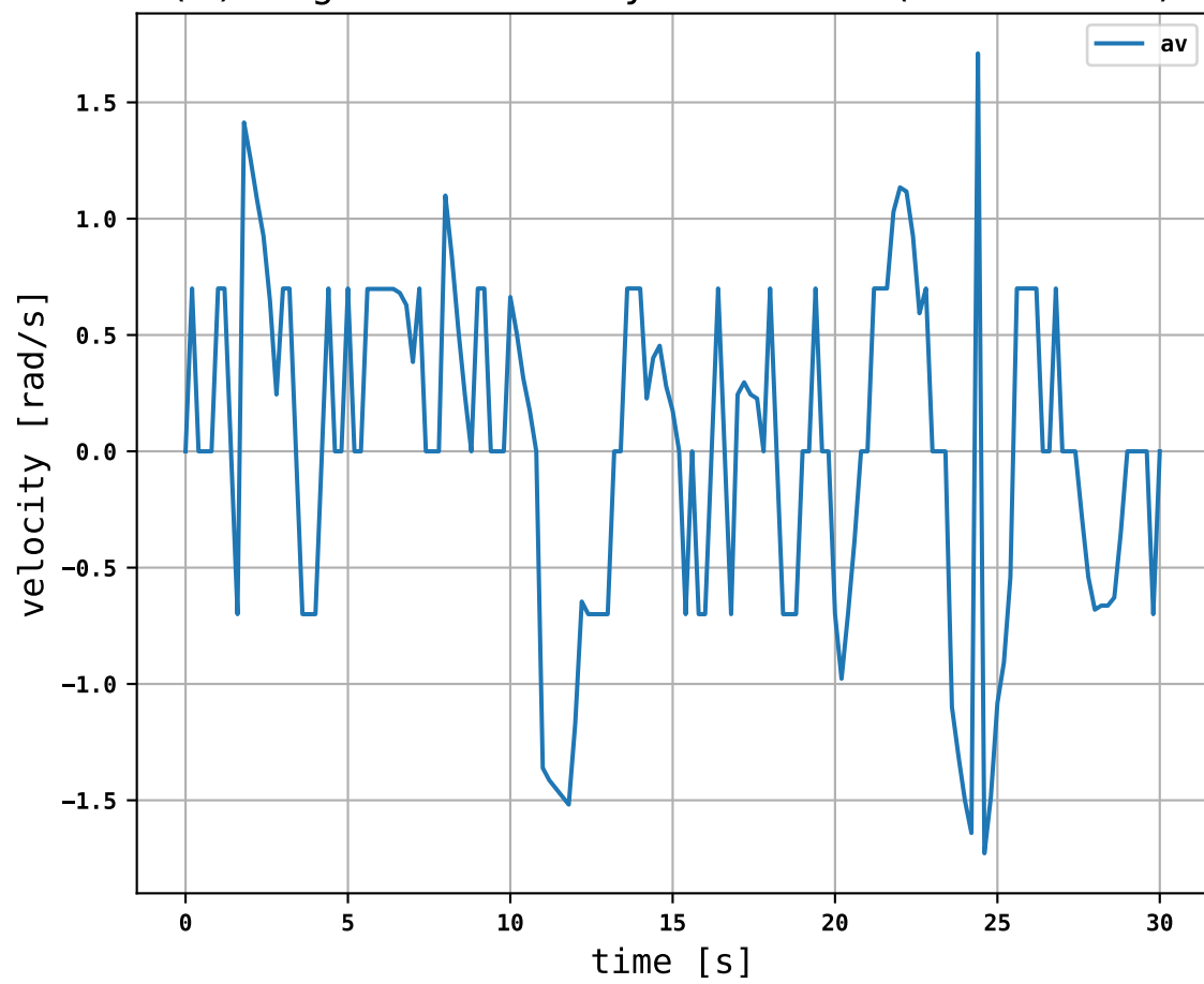
(4) Angular velocity commands (d-modelFMU)
