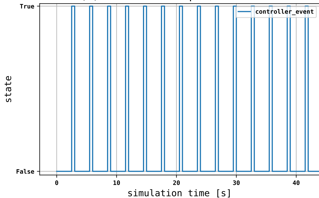
(4) Heater control
