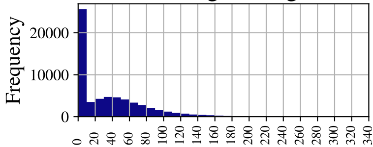
Stress range histogram
