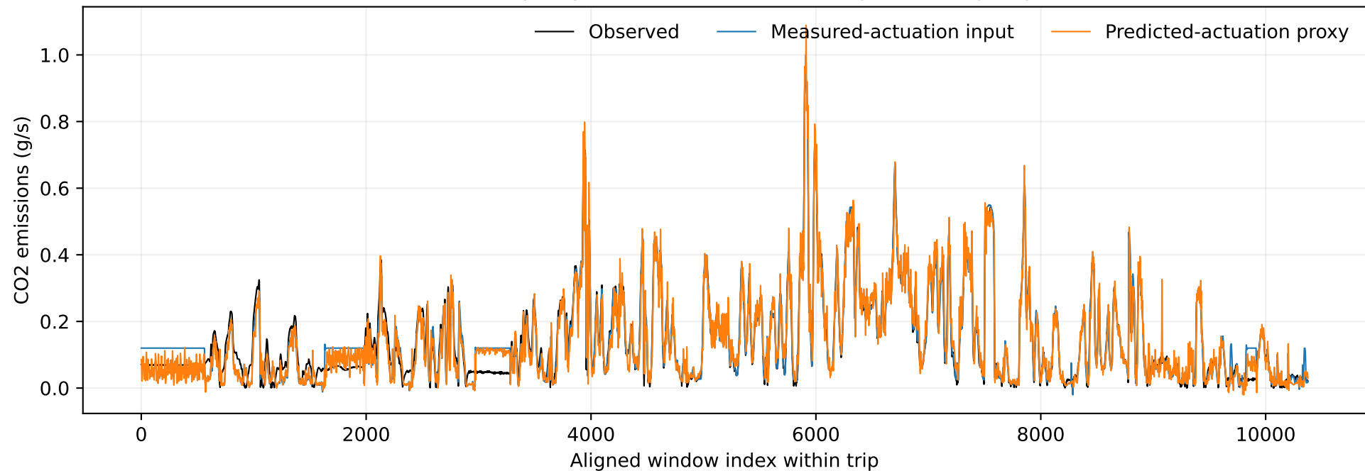
Corrected EV proxy validation - median-length test trip TripB21
