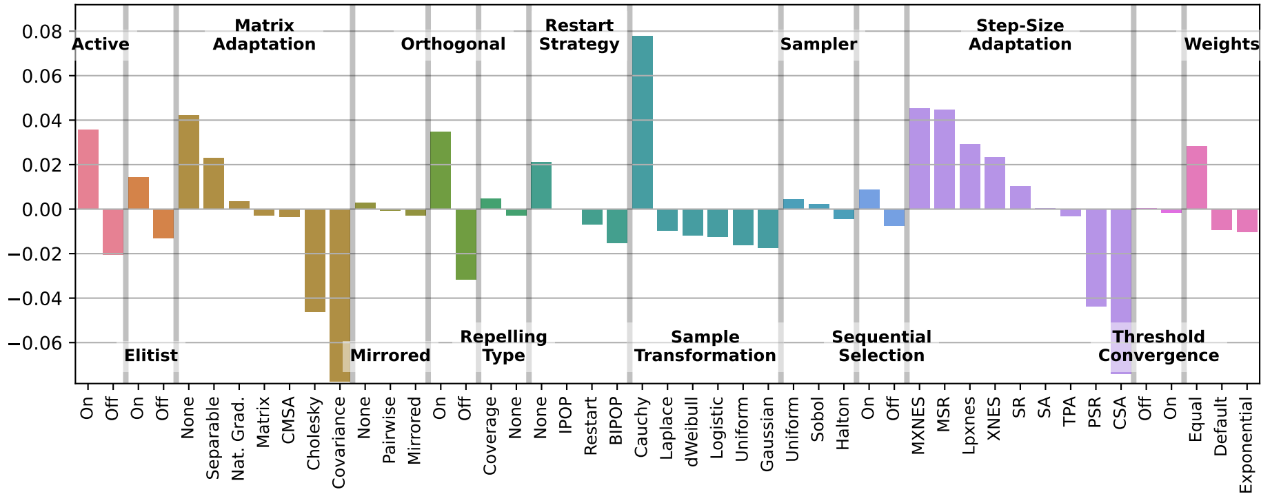
Median SHAP value
